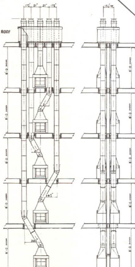
TEN CAT. NO. 3028 FIREPLACES (BACK-TO-BACK, FIVE-STORY) FIREPLACES ARE ON SAME CENTERLINE. TERMINATION ABOVE ROOF IS VIA LOCALLY-CONSTRUCTED CHASE.
