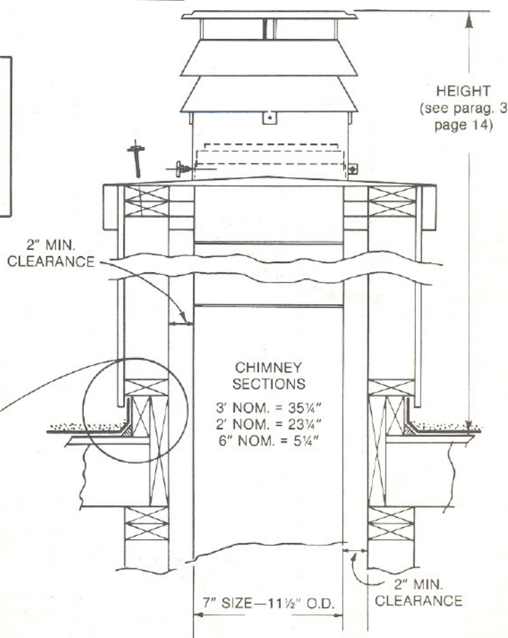
END VIEW
