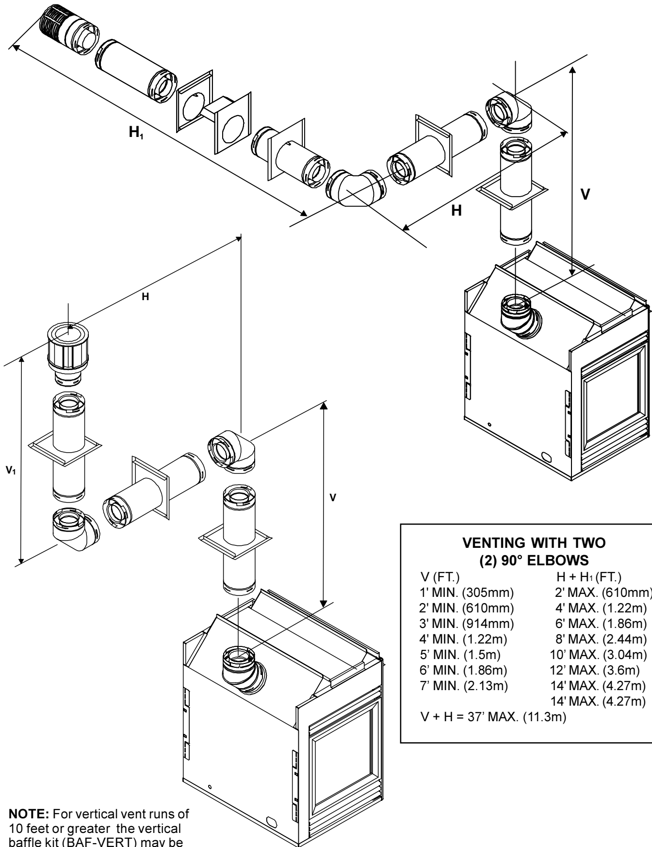
Figure 11. Venting with Two 90° Elbows
