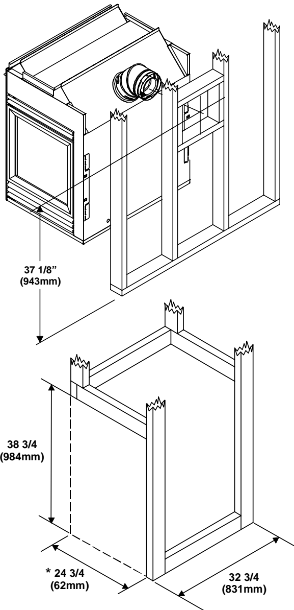
Figure 3. Framing Dimensions
