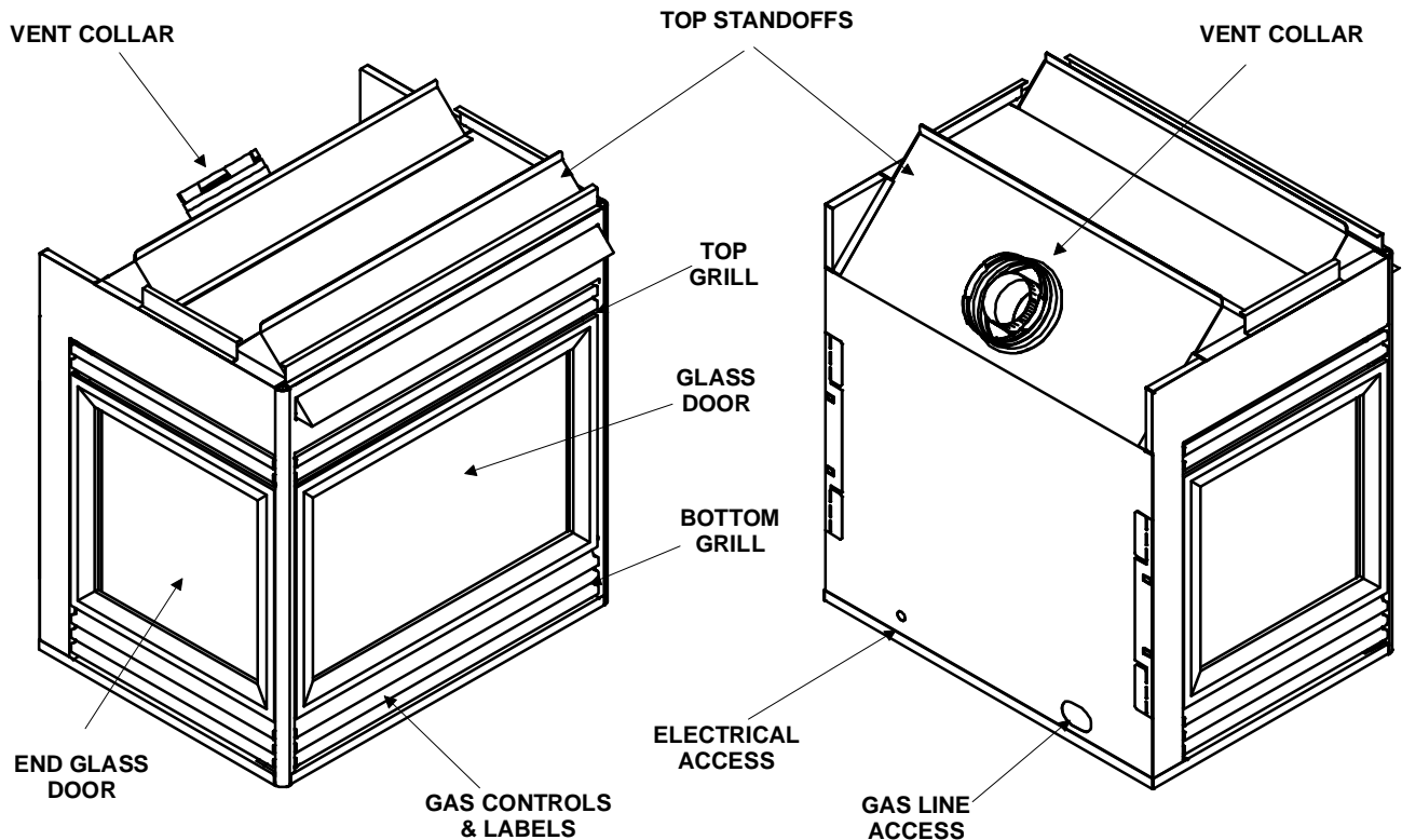
Figure 1. Diagram of the BAY-38HV
