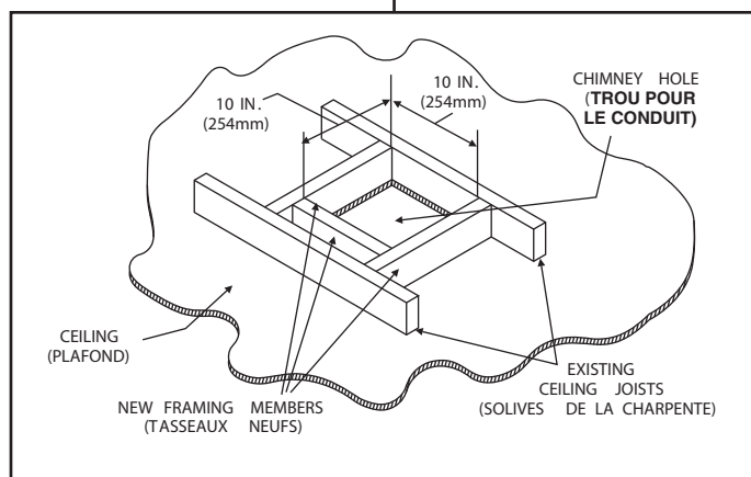
Figure 16. 10" x 10" Hole and New Framing Members
