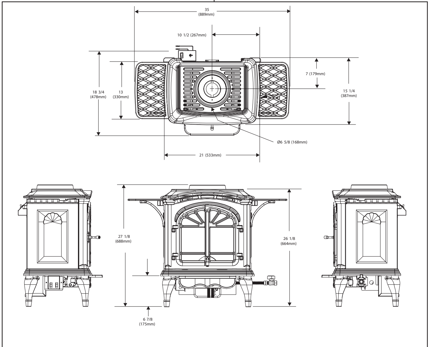
Figure 1. Diagram of the Tiara I
