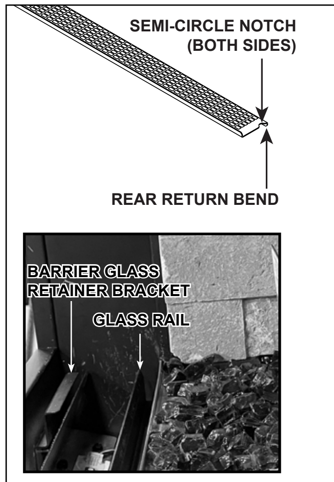
Figure 4.9 Install Transition Media Tray
