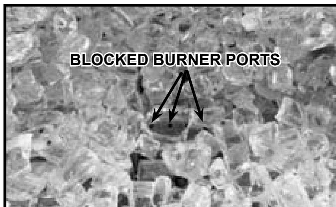
Figure 11.9 Blocked Burner Ports
