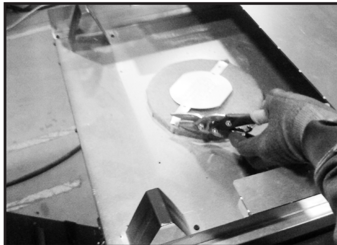
Figure 6.3 Cut the metal retaining band and fold the sides out.
