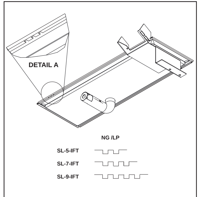
Figure 9.2 Burner Identification
