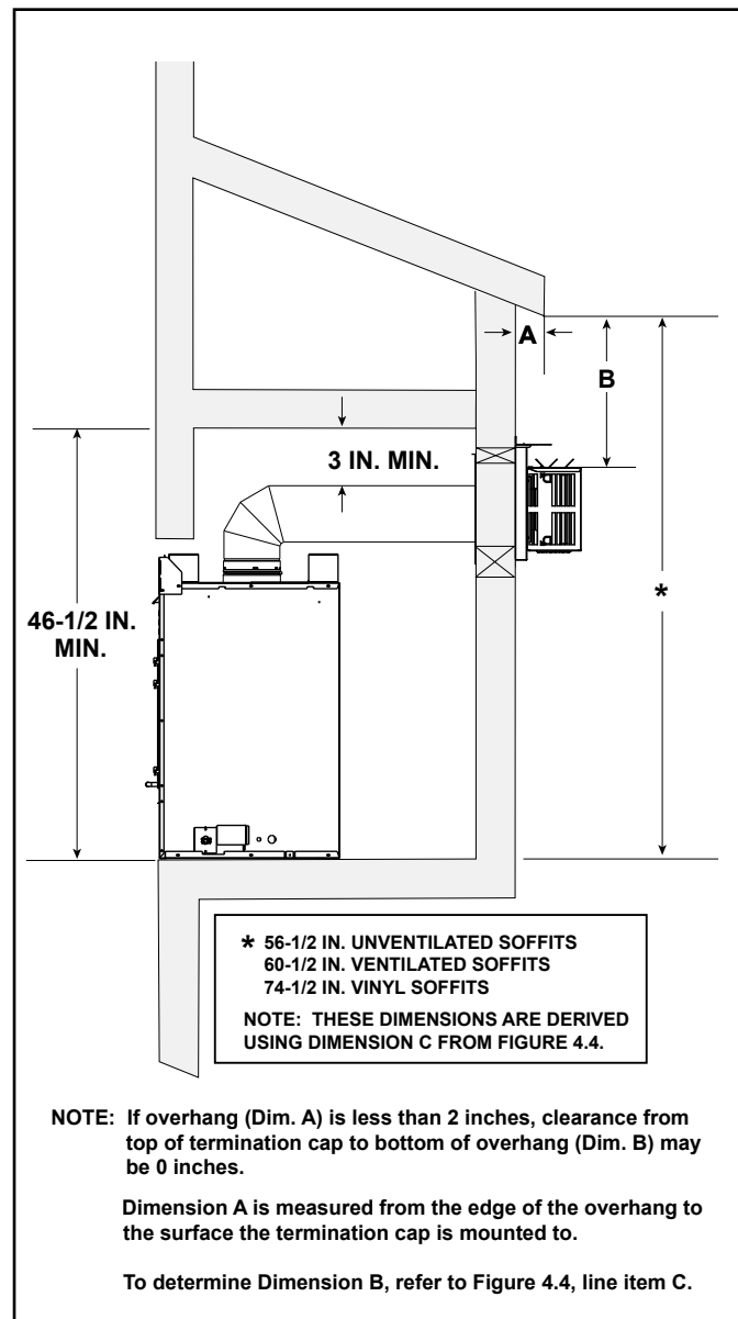
Figure 3.6 Exterior Chase - Minimum Height Requirements
