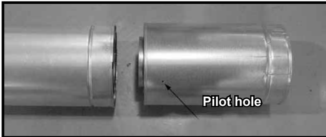
Figure 7.6 Slip Section Pilot Holes
