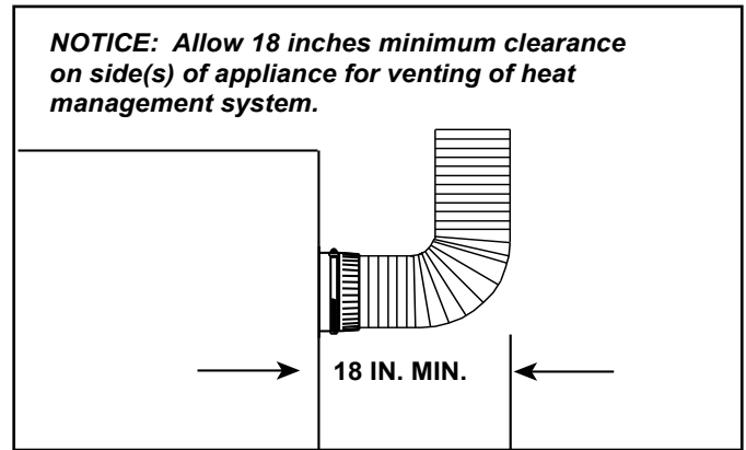
Figure 3.3 Clearance for Heat Management System
