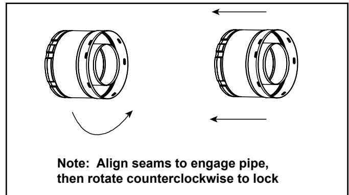
Figure 7.5 Adding Venting Components
