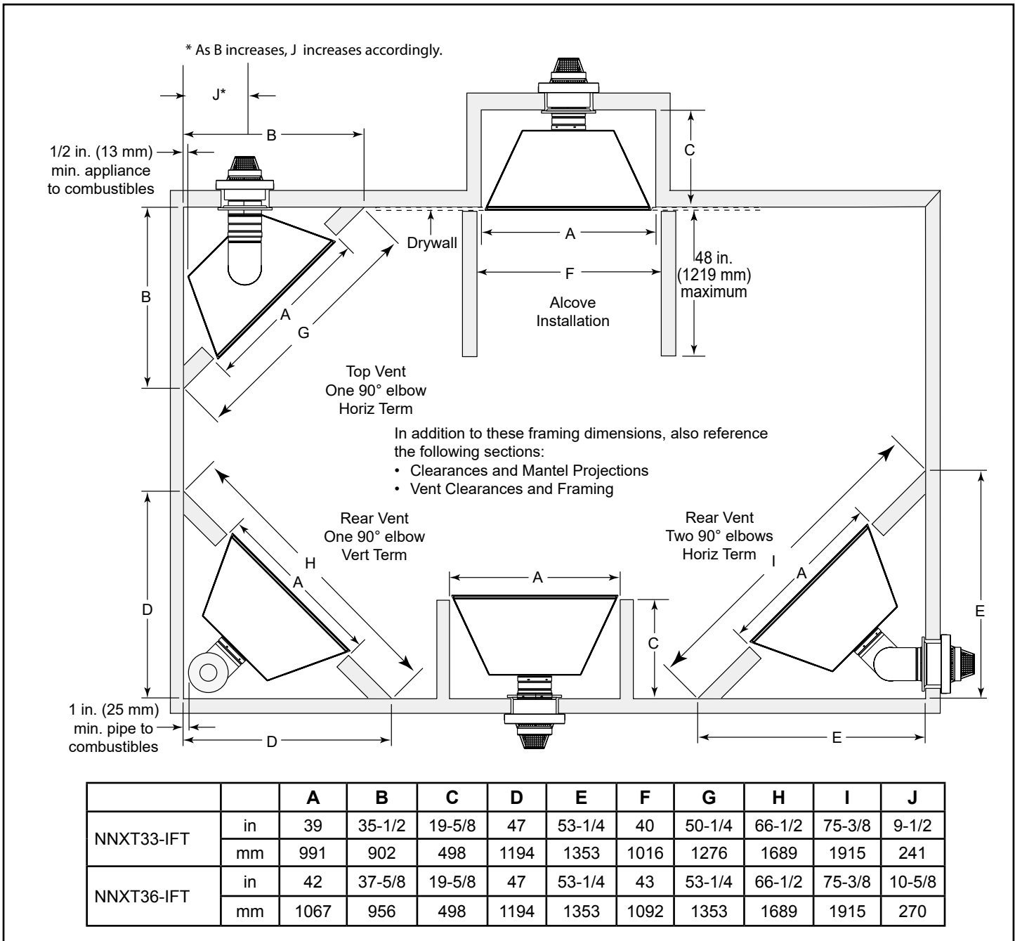
Figure 3.4 Appliance Locations
