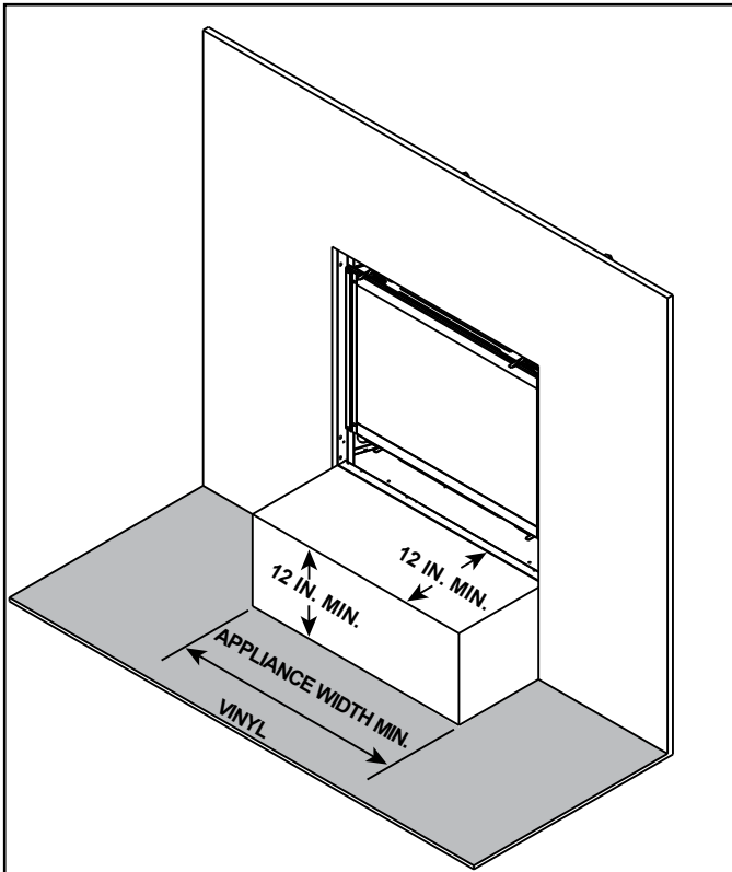
Figure 3.7 Vinyl Flooring Recommendations
