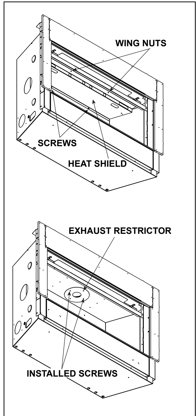
Figure 4.17 Installing Restrictor
