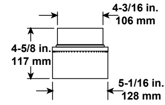
DVP-2SL Adapter
