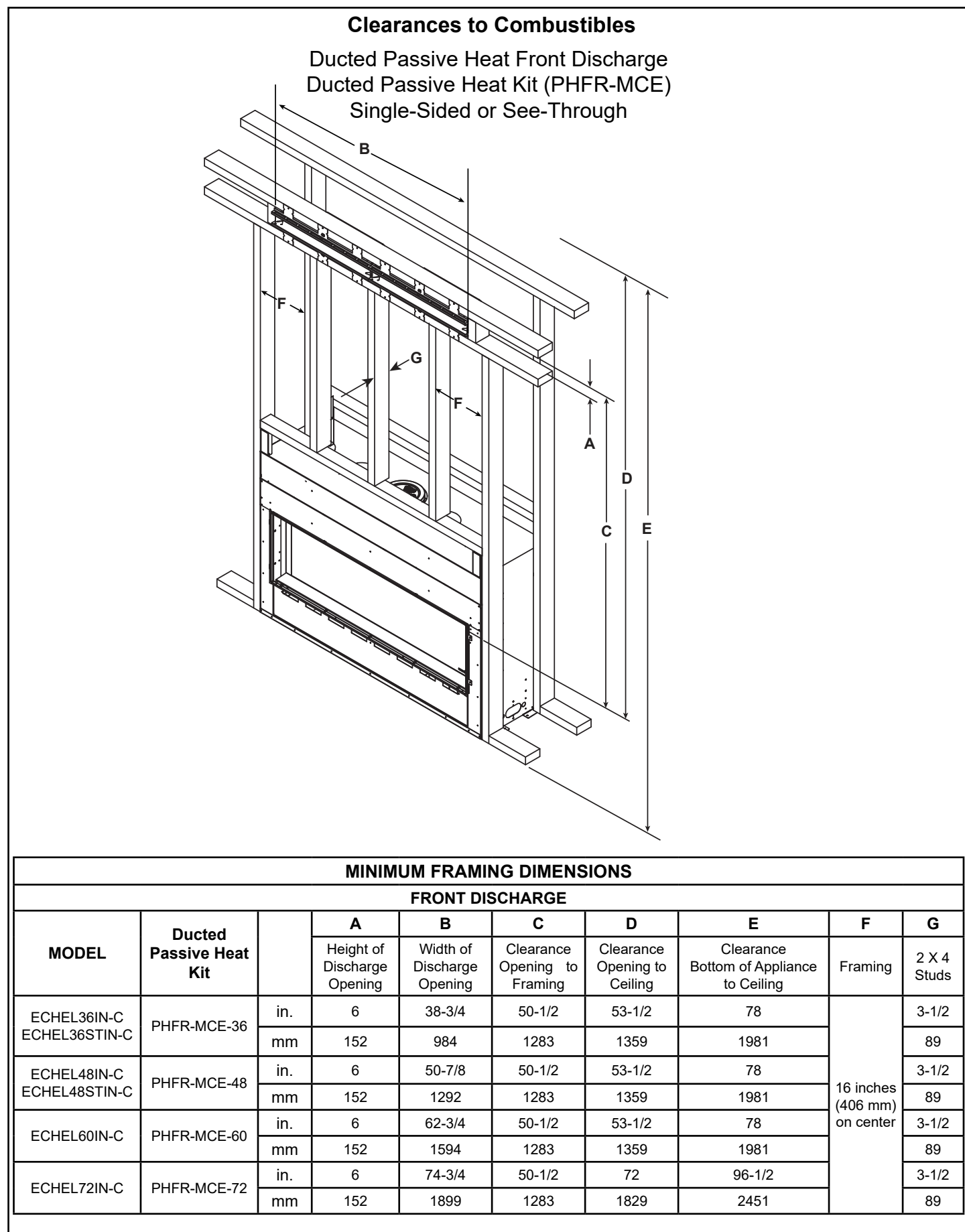
Figure 3.14 Clearances to Combustibles - Ducted Passive Heat Front Discharge
