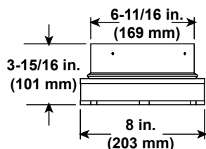
SL-2DVP Adapter
