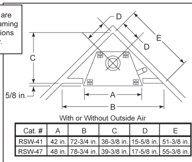
Figure 4 Corner Installation
