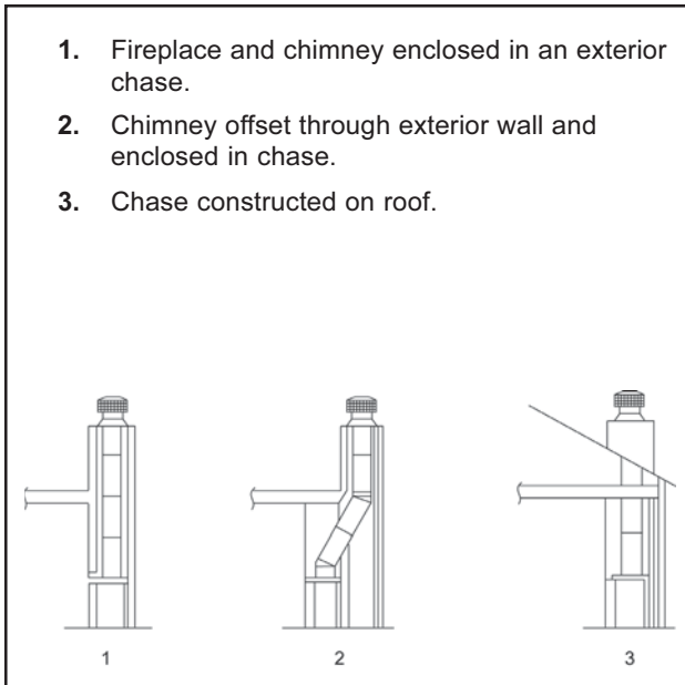
Figure 20 - Chase Constructions
