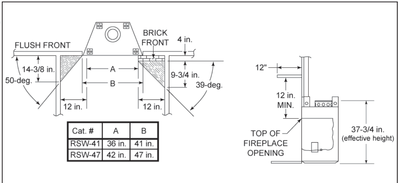
Figure 6 - Sidewalls and Surrounds
