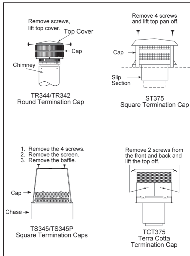
Figure 28 Chimney & Termination Cap Cleaning
