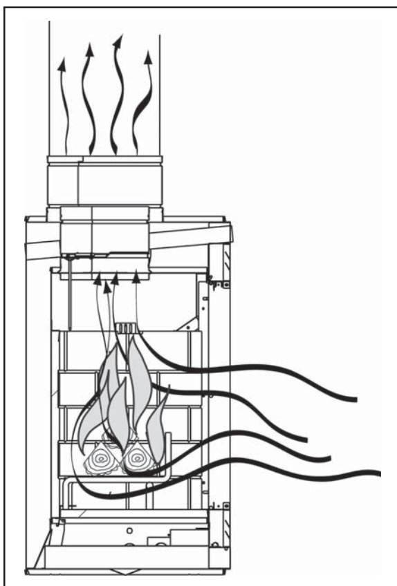
Figure 27 - Flue Draft
