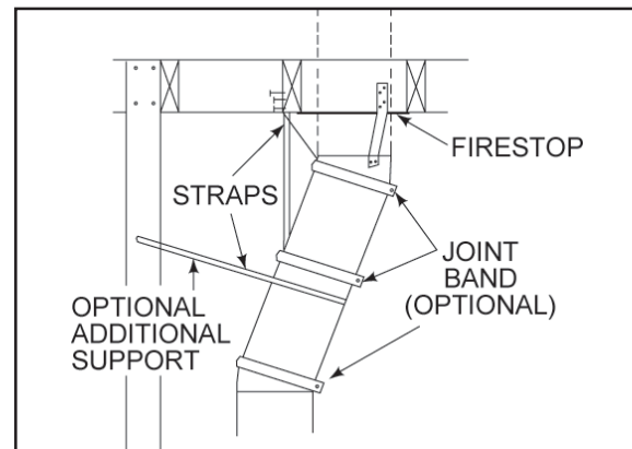
Figure 13 - Offset/Return with Stabilizer
