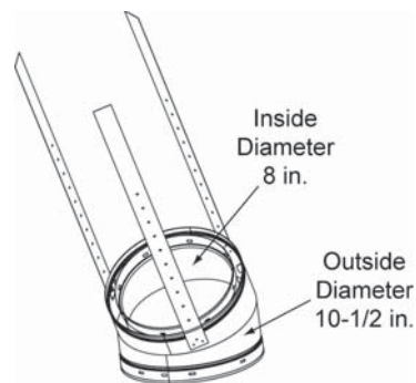
SL330 - Offset/Return
