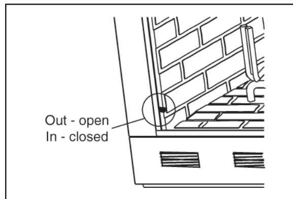
Figure 15 - Air Kit Handle Location
