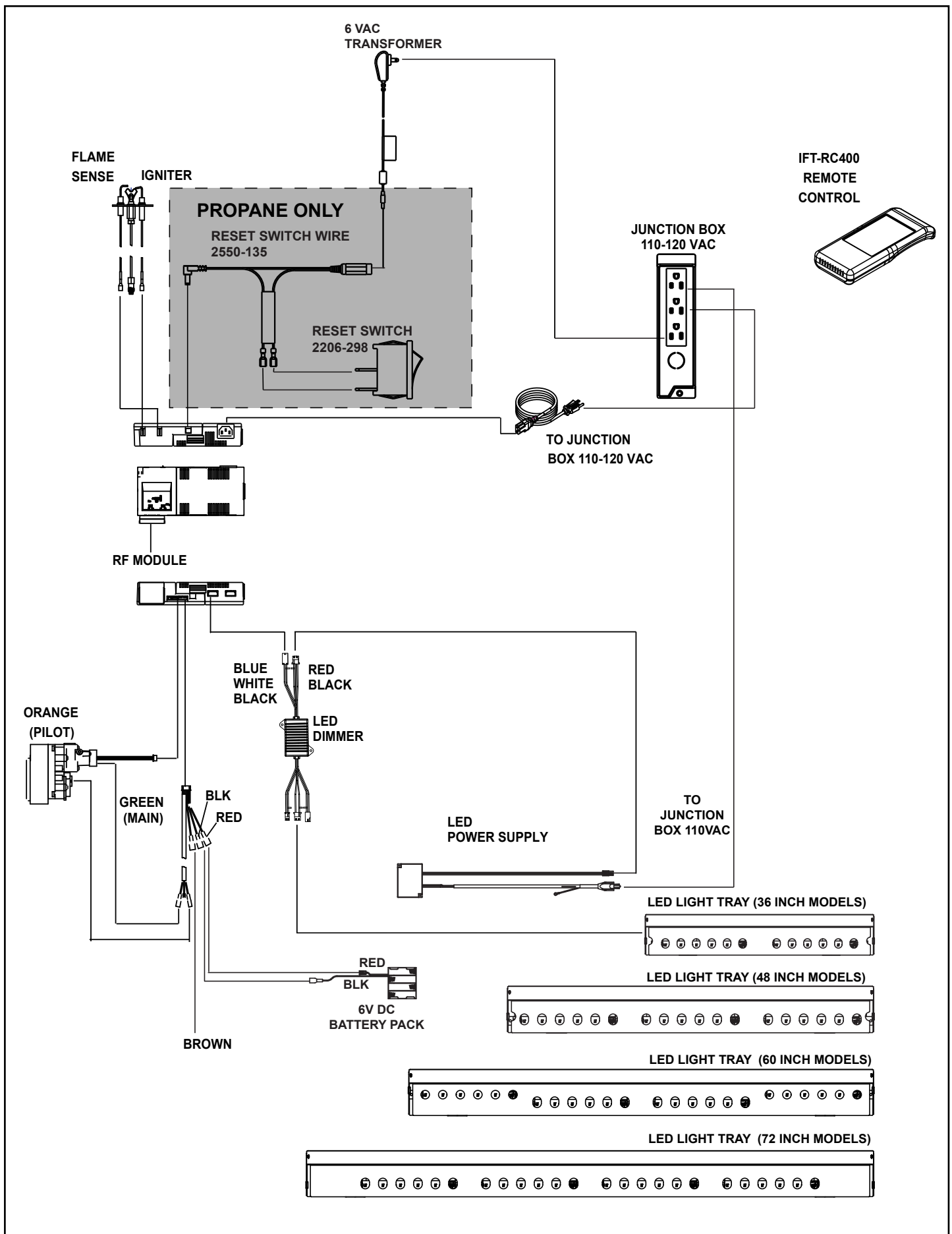
Figure 8.3 IntelliFire Touch Wiring Diagram
