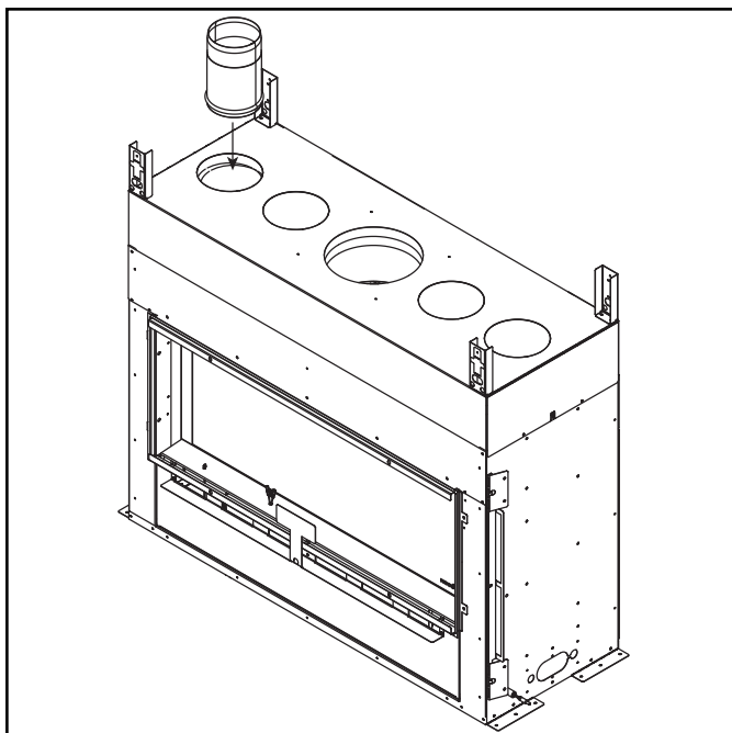
Figure 6.5 Heat-Zone-Gas Linear Adapter Collar
