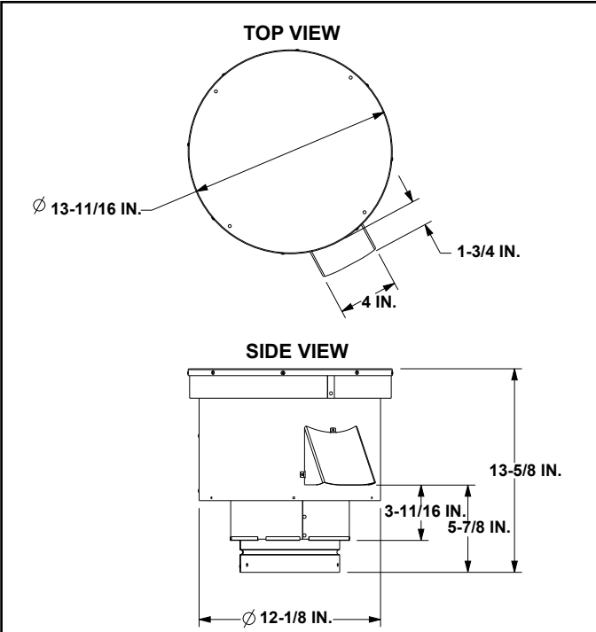
Figure 12.5 Vent Components
