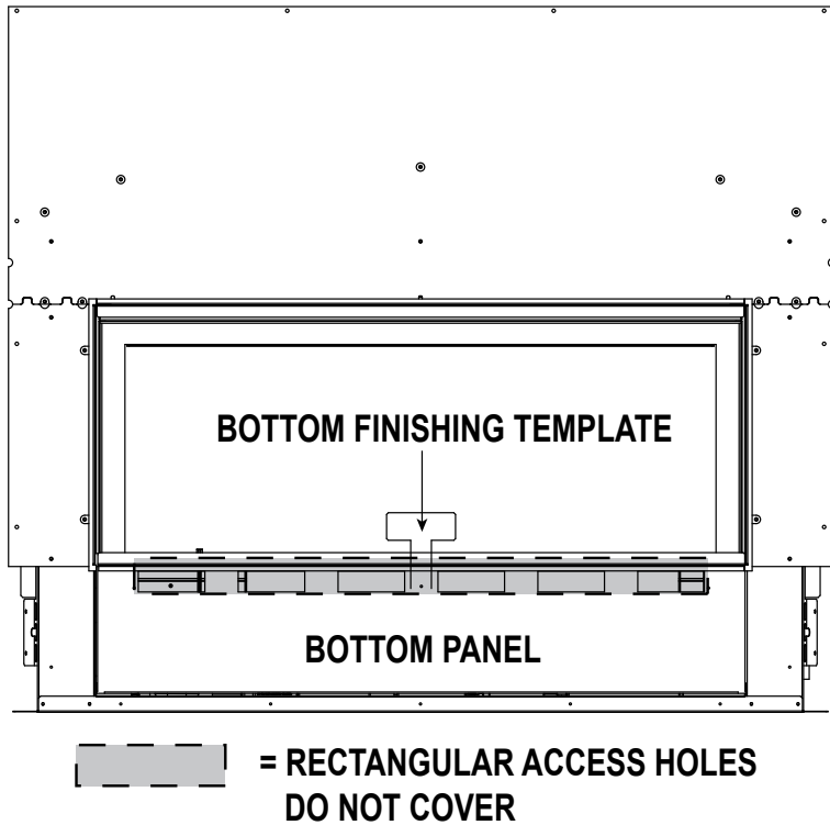
Figure 10.9 Non-Combustible Finishing Material Diagram for 0-1 Inch Thick Overlap Fit Method (Quattro/Forge)
