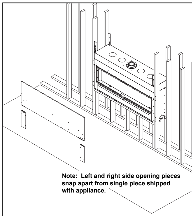
Figure 6.9 Install Factory-Included Non-Combustible Facing Material
