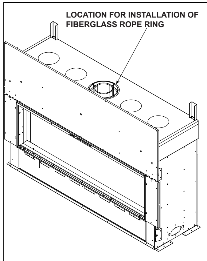
Figure 6.2 Location of Fiberglass Rope Ring
