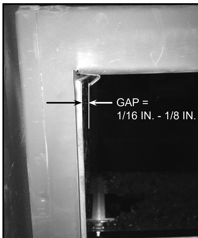
Figure 6 Gap Between Tab and Side Glass Panel: 1/16 IN. - 1/8 IN.
