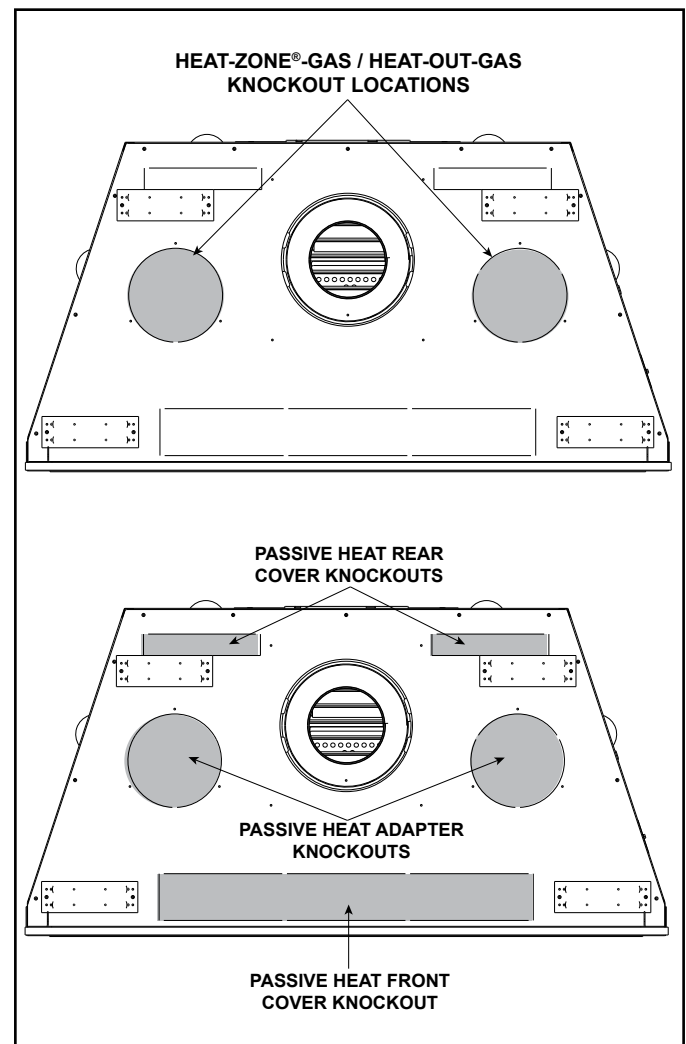
Figure 6.4 Heat Management Knockout Locations
