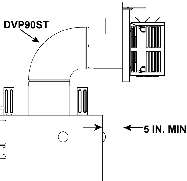
Figure 3.11 DVP-TRAP1 Exception (2 x 4 Construction)
