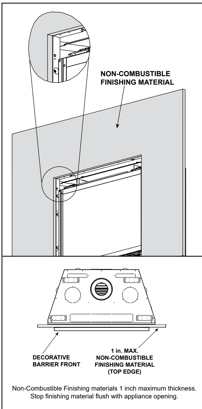
Figure 10.14 Non-Combustible Finishing Material 1 Inch Thick or Less - Overlap Fit Fronts
