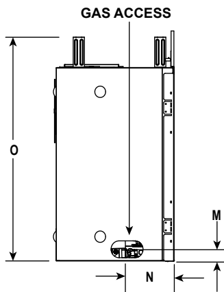
Appliance Dimensions Table - 6KX
