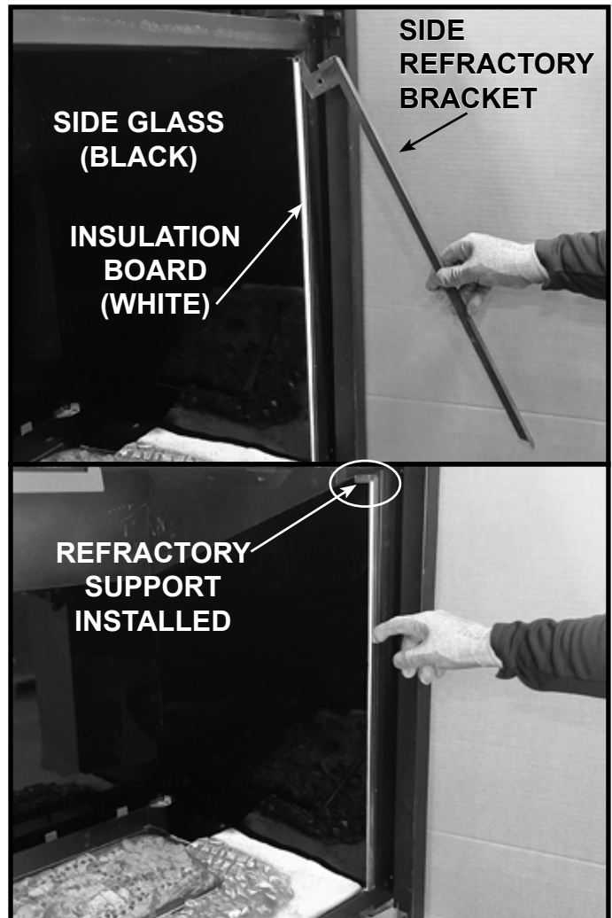
Figure 11.18 Install Side Refractory Bracket with Side Insulation Board and Side Glass Panel
