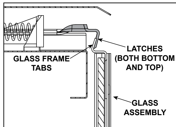
Figure 11.29 Fixed Glass Assembly
