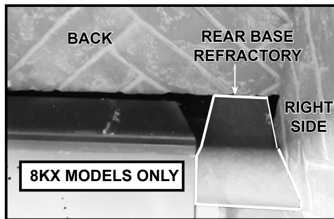
Figure 11.7 8KX Models Only: Rear Base Refractory Piece Installed (Right Side Shown)
