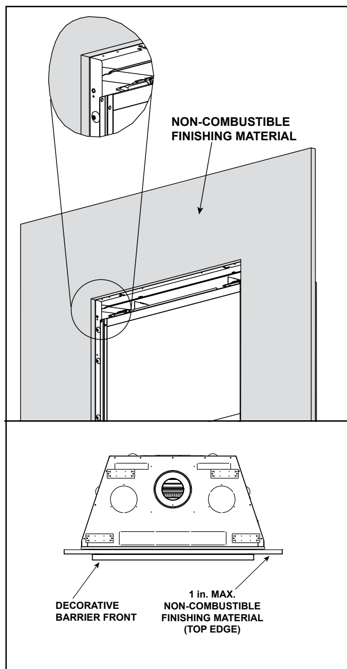
Figure 10.14 Non-Combustible Finishing Material 1 Inch Thick or Less - Overlap Fit Fronts
