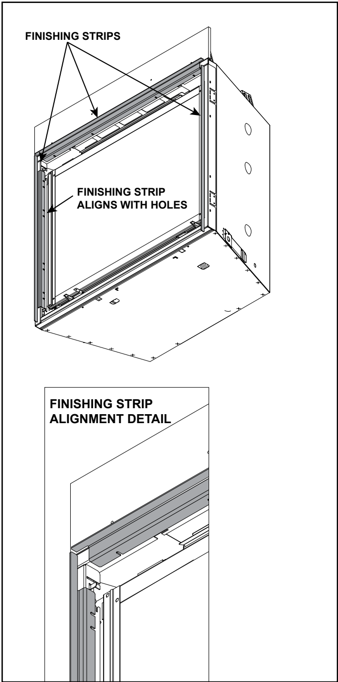
Figure 10.17 Install Finishing Strips
