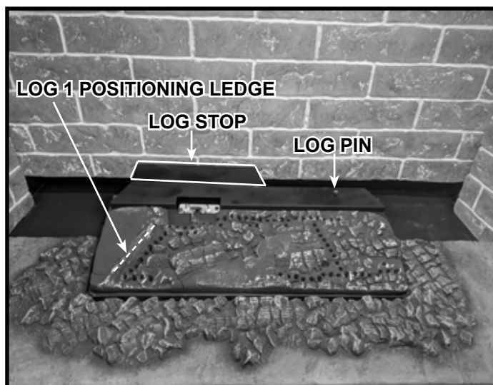
Figure 2 Log Location Features
