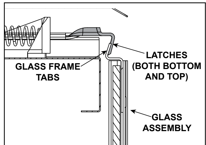
Figure 11.14 Fixed Glass Assembly
