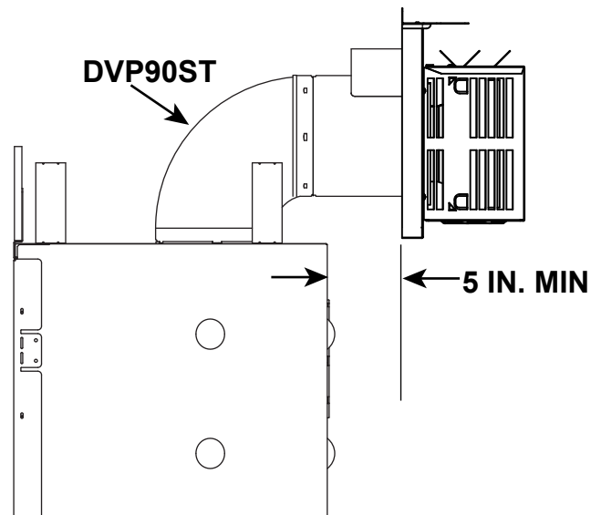
Figure 3.11 DVP-TRAP1 Exception (2 x 4 Construction)
