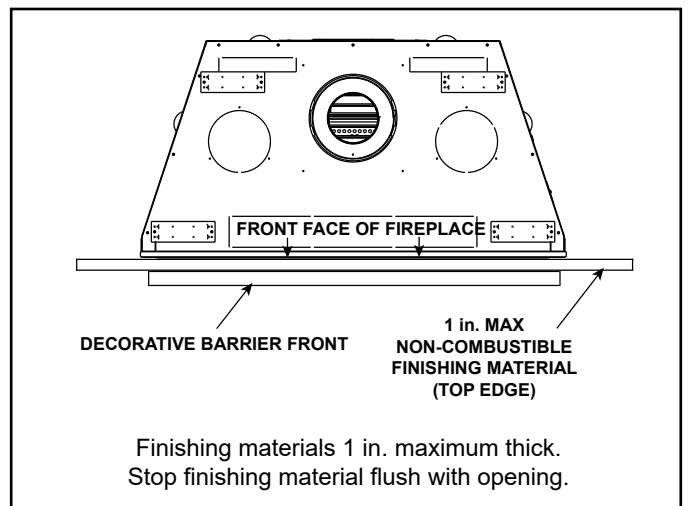
Figure 10.13 Overlap Fit Decorative Barrier Front
