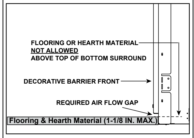
Figure 10.3 Required Air Flow Gap
