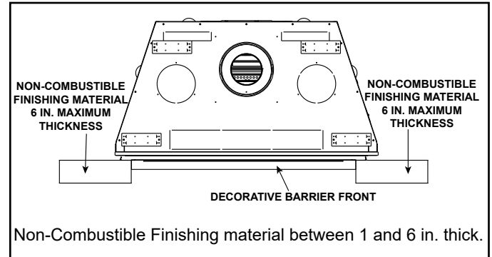
Figure 10.12 Inside Fit Decorative Barrier Front
