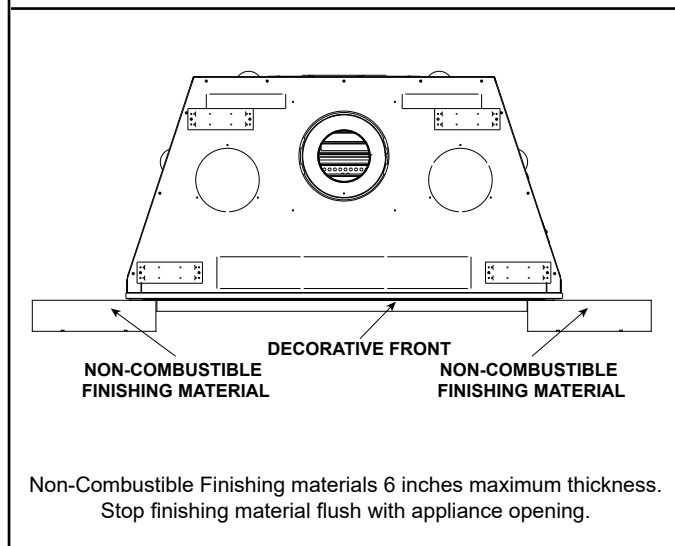
Figure 10.15 Inside Fit Method
