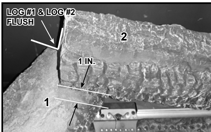
Figure 4.B Log #2 Placement (8K-NG, 8K-LP and 6KX-LP Appliance Models Only)
