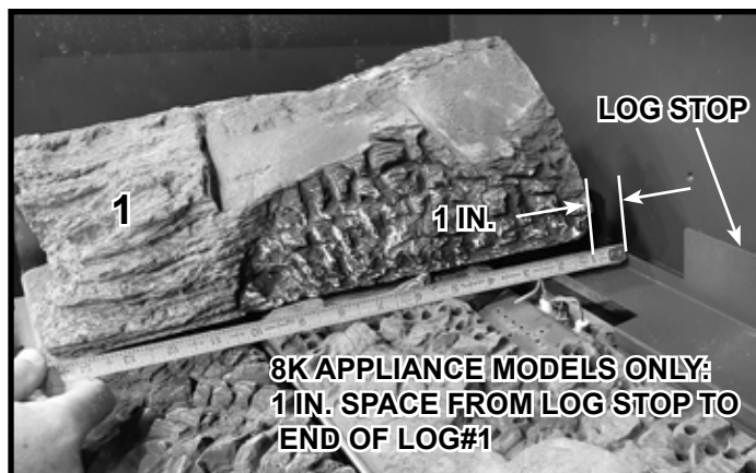
Figure 3.B Log #1 Clearance to Log Stop (8K Appliance Models Only)
