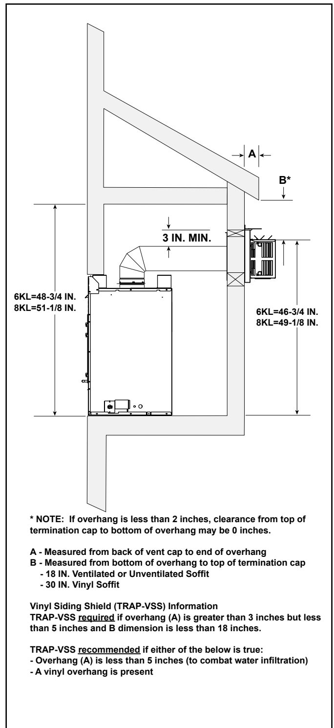
Figure 3.16 Exterior Chase - Minimum Height Requirements
