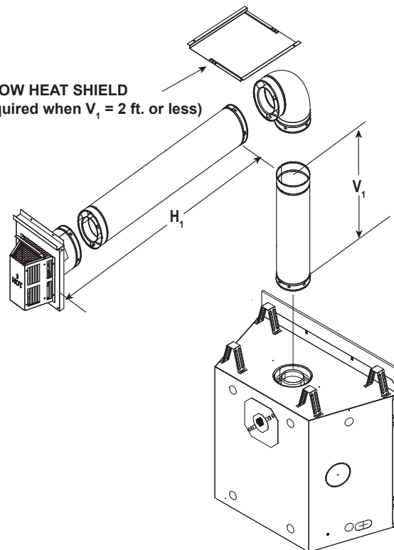
Figure 5.2 Elbow Heat Shield Requirements
