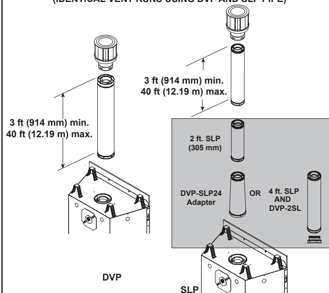
Figure 4.10 DVP-SLP24 Adapter
