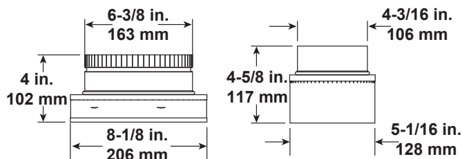
DVP-2SL Adapter
