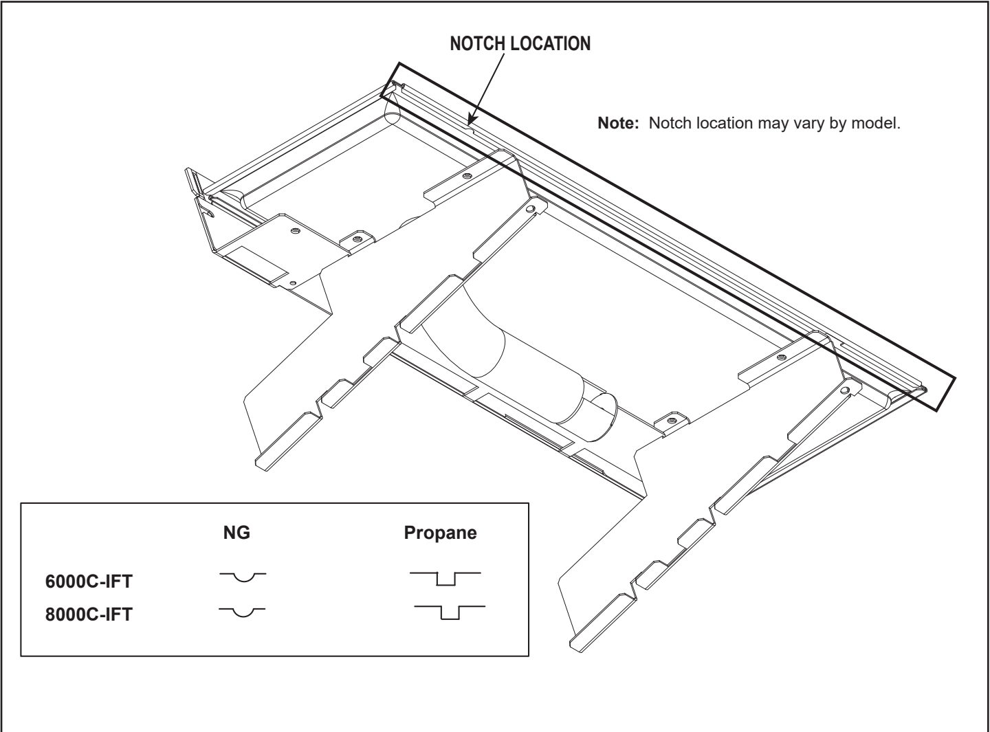
Figure 4.6 Burner Identification
