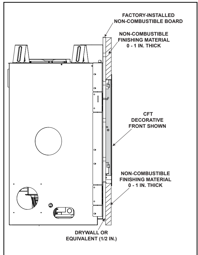
Figure 10.8 Overlap Fit Method (CFT and Martini Decorative Fronts)
