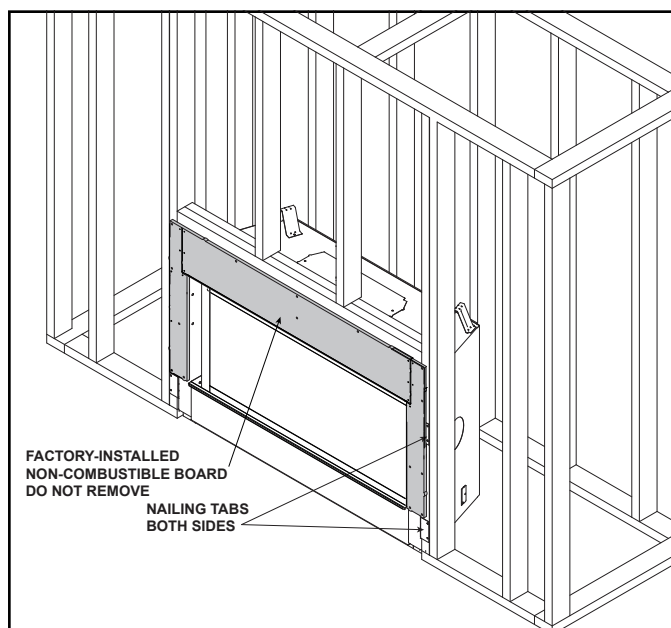
Figure 6.5 Proper Positioning, Leveling And Securing Of Appliance
