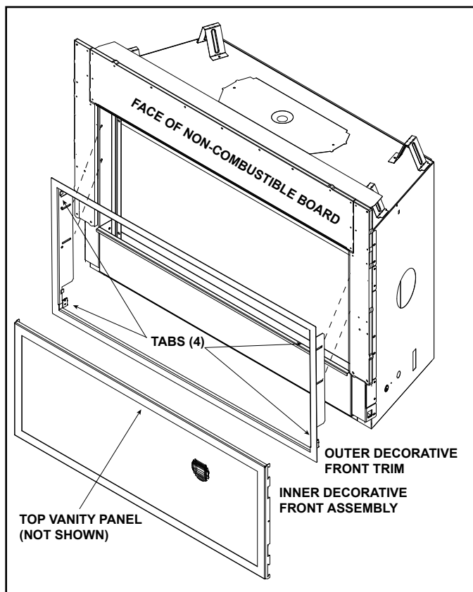
Figure 10.11 CFT Front Installation With Outer Decorative Front Trim
