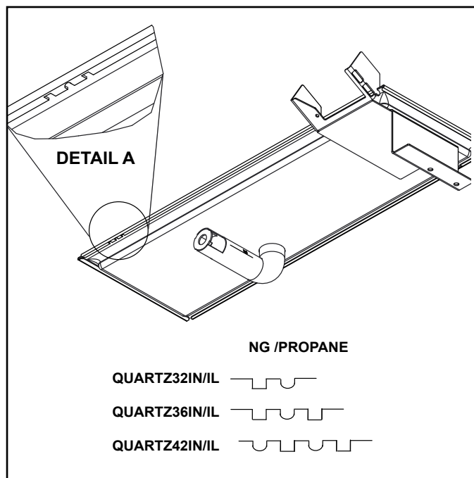
Figure 9.2 Burner Identification
