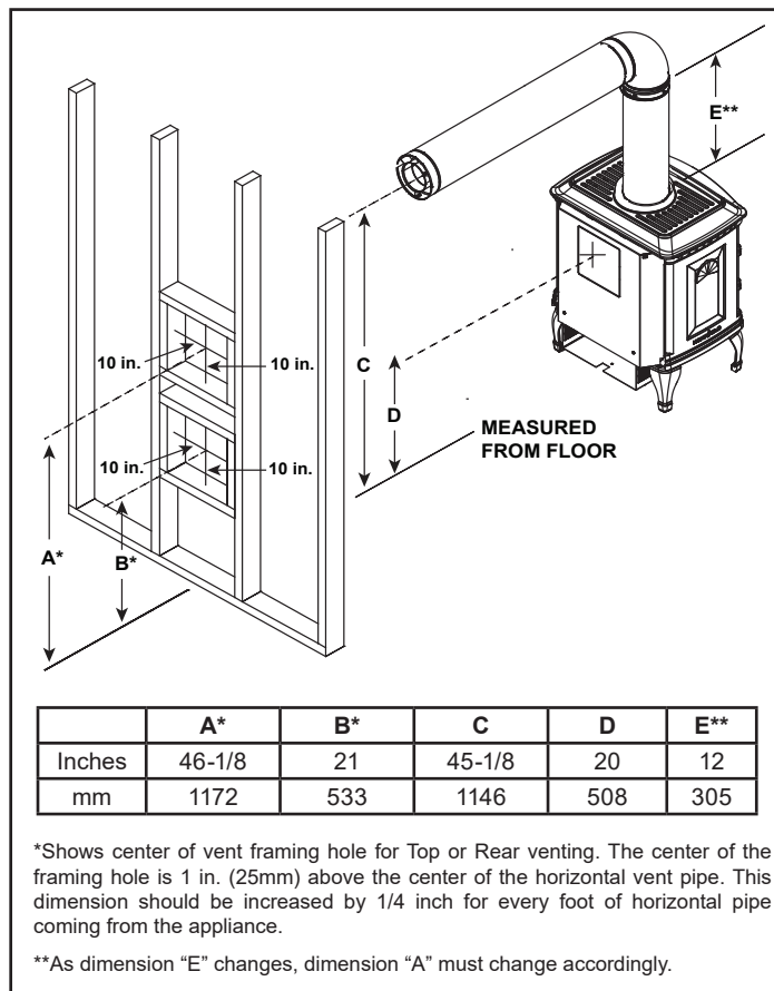
Figure 5.2 - Wall Penetration
