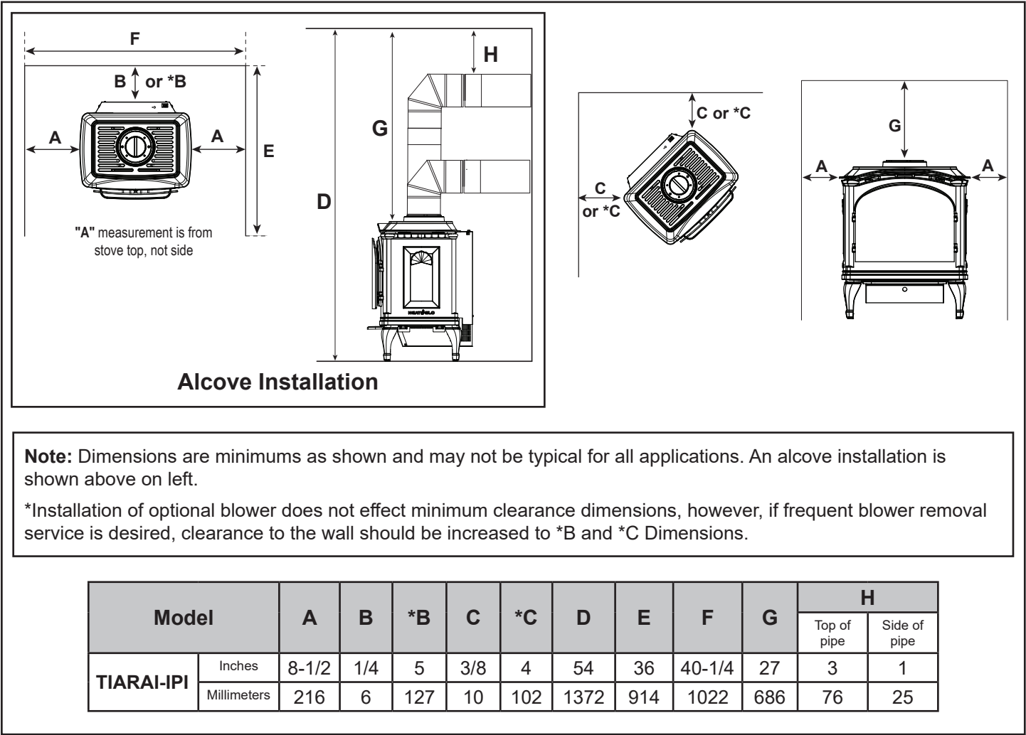
Figure 3.2 - Appliance Locations
