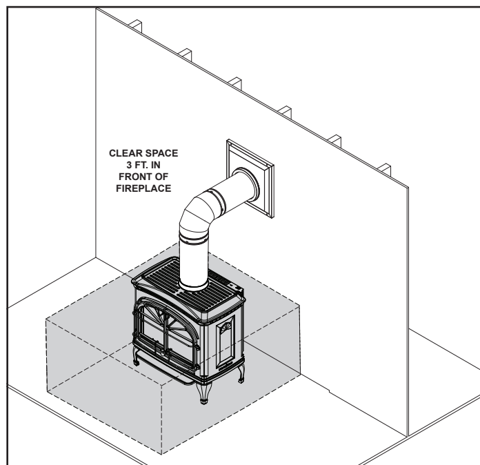
Figure 3.1 Clear Space
