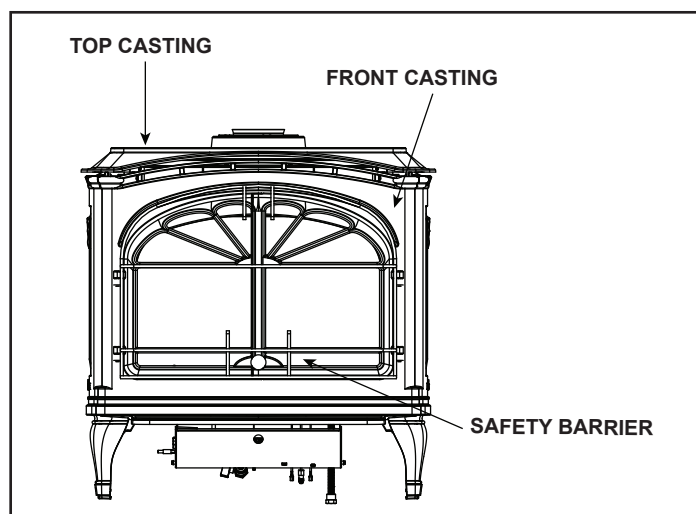
Figure 4.1 Remove Casting
