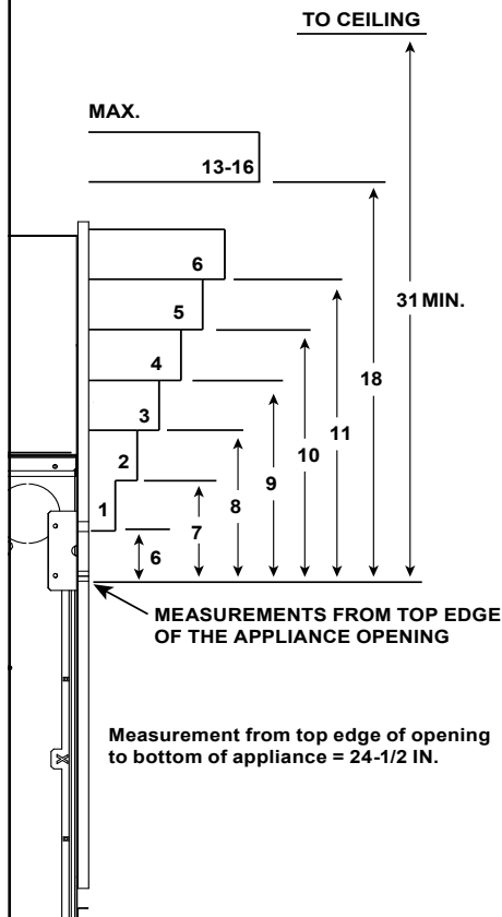
Figure 10.14 Minimum Vertical and Maximum Horizontal Dimensions of Non-Combustibles - Overlap Fit Finishing
