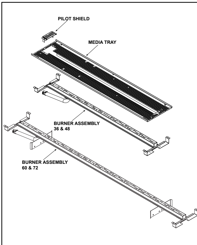
Figure 9.3. Media Tray with Burner and Pilot Shield
