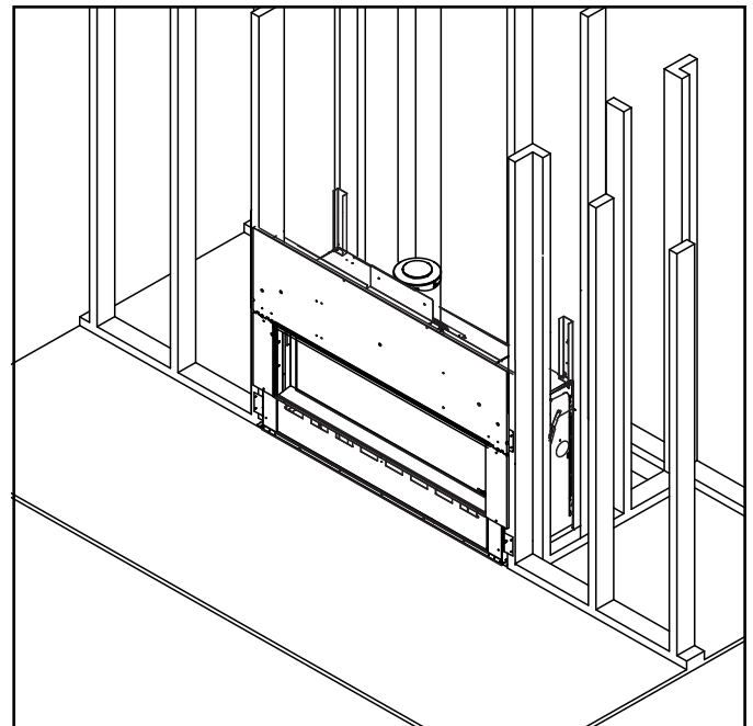
Figure 3.12 Floor Protection
