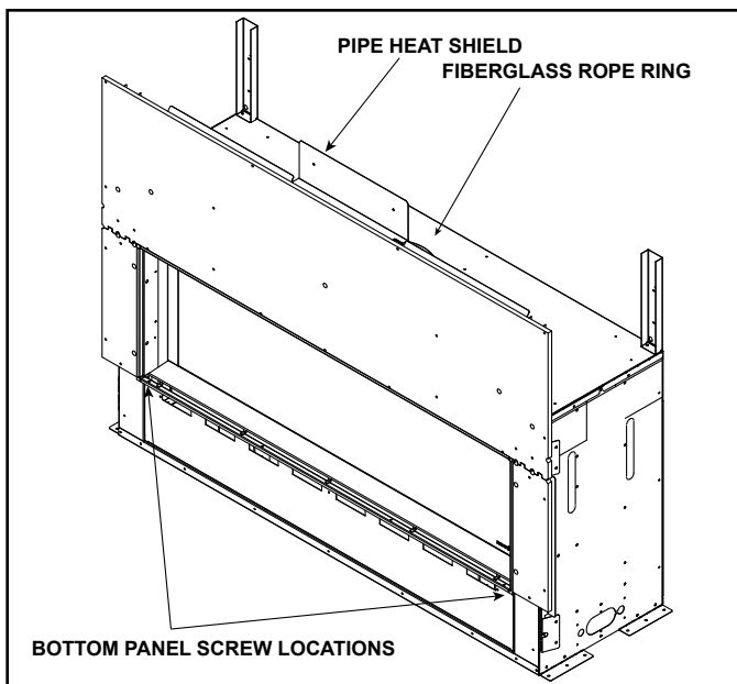
Figure 6.3 Location of Fiberglass Rope Ring
