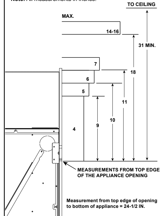
Figure 10.15 Minimum Vertical and Maximum Horizontal Dimensions of Non-Combustibles - Inside Fit Finishing
