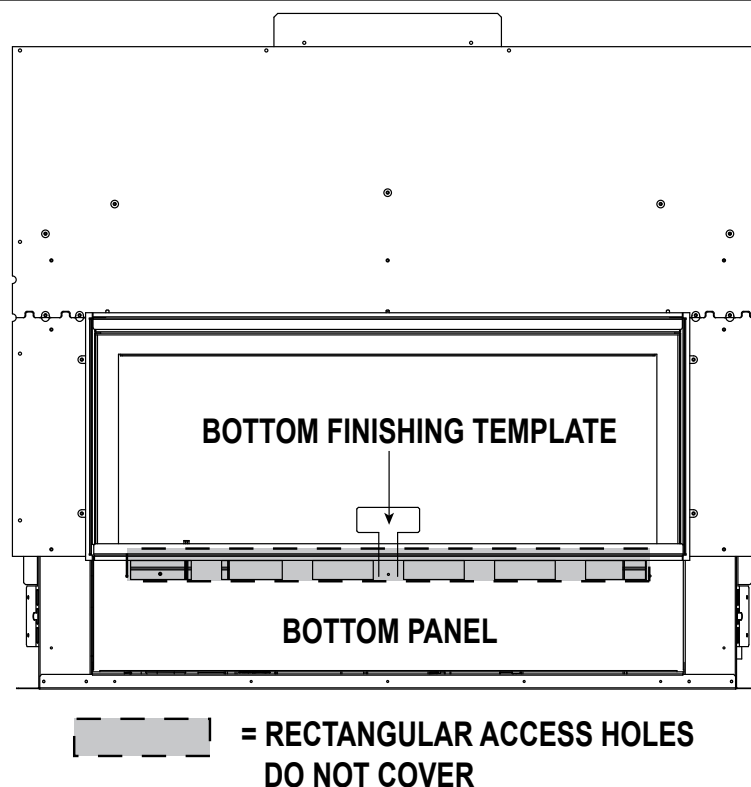
Figure 10.9 Non-Combustible Finish Material Diagram for 0-1 Inch Thick Overlap Fit Method (Quattro/Forge)
