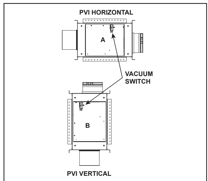
Figure 4.20 Vacuum Switch Location - Horizontal/Vertical Orientation
