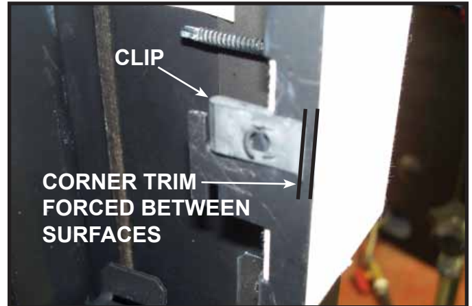
Figure 8. Clip Location.
