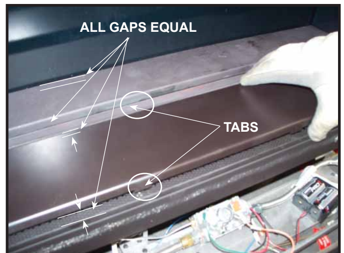
Figure 5. Placing Base Pieces.
