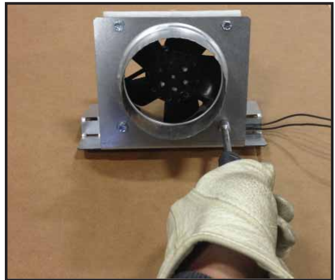
Figure 8.18 Removal of Mounting Bracket from Blower
