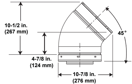
DVP45 (45° Elbow)
