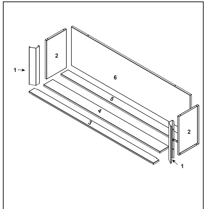
Figure 18. Service Parts Diagram.
