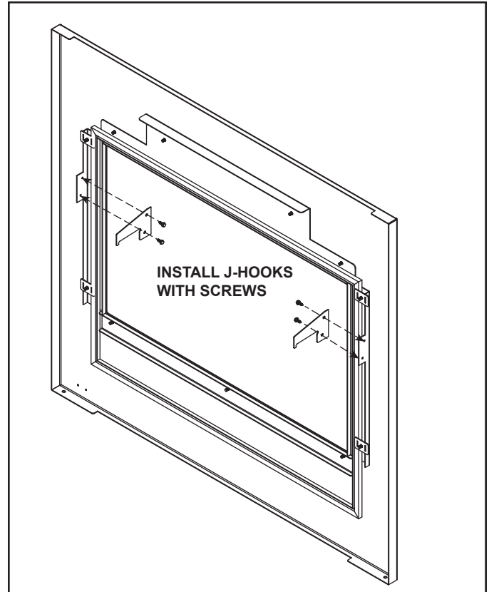
Figure 1. Install J-Hooks to Brackets(?)
