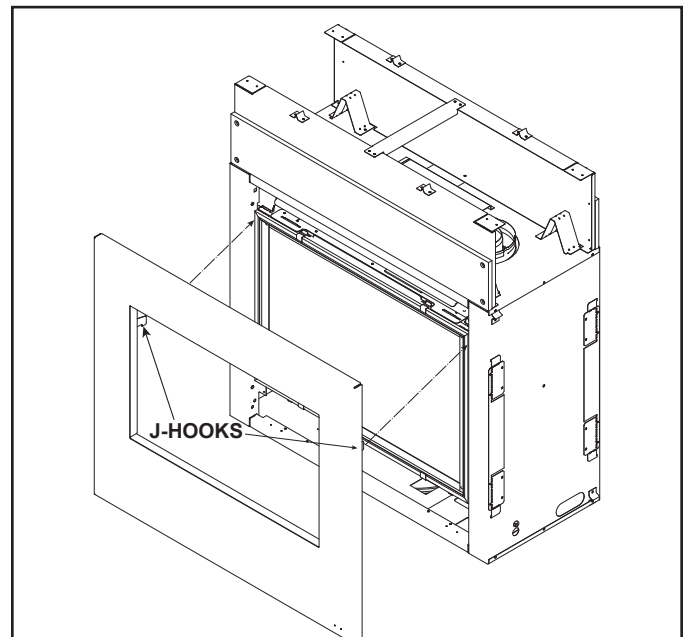
Figure 2. Installing Door on Appliance.
