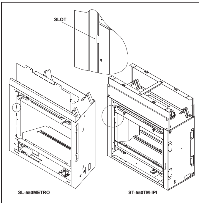
Figure 3. Slot Location
