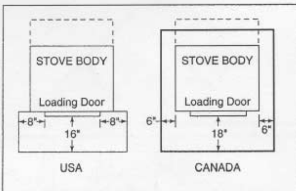
Figure 4 Floor Protection
