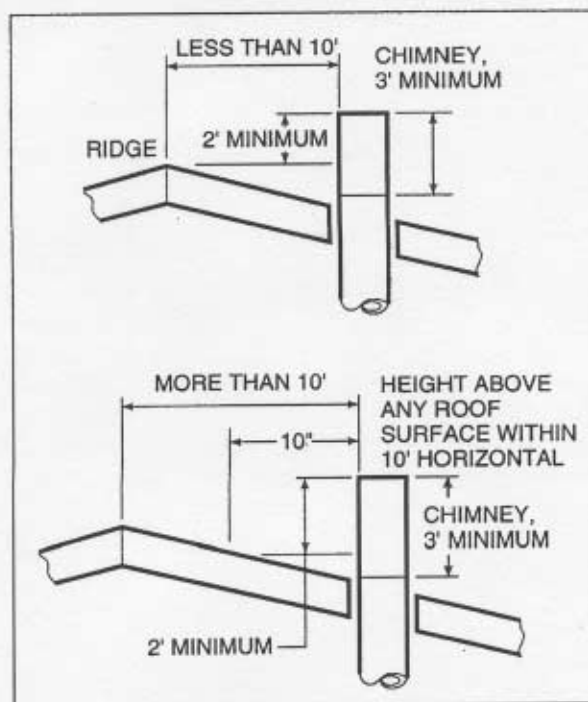
Figure 6 Chimney Height
