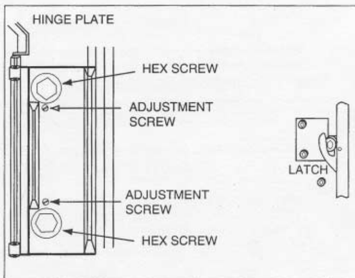
Figure 20 Door Adjustment
