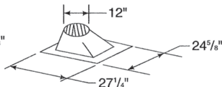
6/12 to 12/12 Pitch RF571
