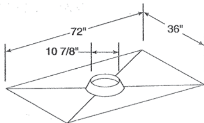
CT56 CHASE TOP
