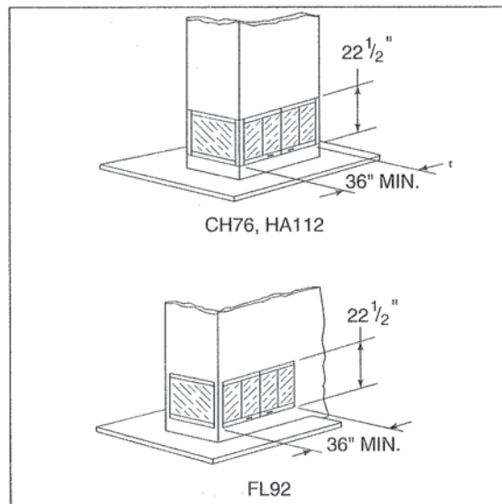
Figure 3 Non-combustible Facing
