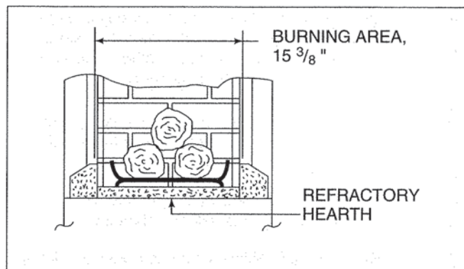
Figure 22 Sectional View of Fireplace
