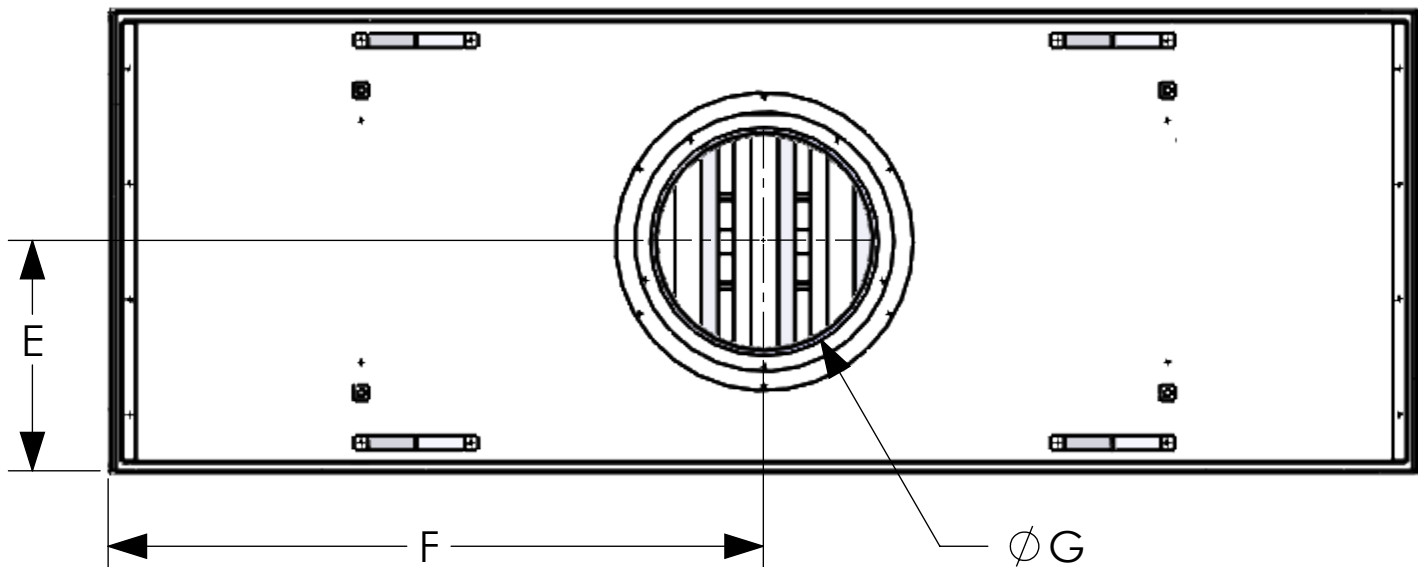
CUSTOM CONFIGURATION: NATURAL VENT, NO DECORATIVE LEDGE
