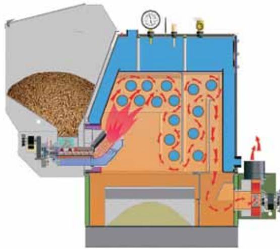
This cut away shows air flow and the Patented Pellet Pro Feeder System at work in the PB105.
