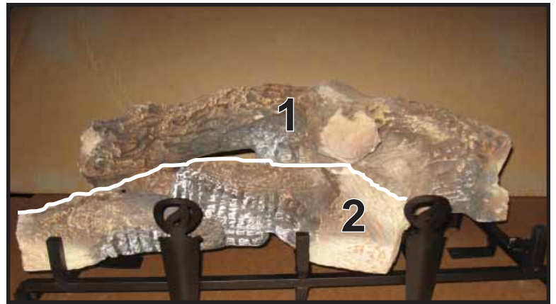
LOG NUMBER 2 (SRV768-704): Position log #2 onto grate such that tab C fits into the slot on the bottom surface of the log. The right side of the log rests between the front grate tine and locating tine E. The cutout on the log should contact the corresponding tine.
