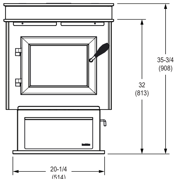
Figure 8.2- Front View
