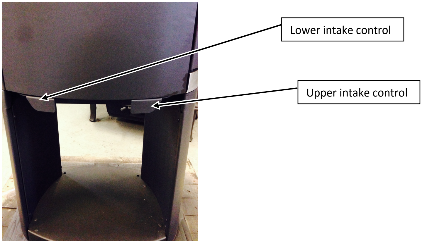
Fig. 11.1: Air Control
