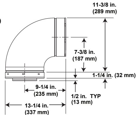
DVP90ST (90° Elbow)
