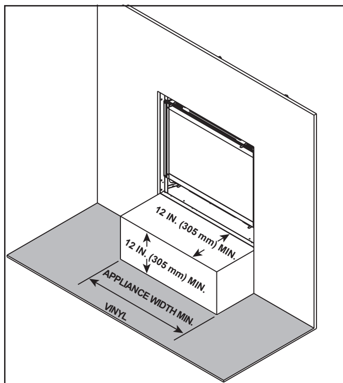
Figure 3.5 Vinyl Flooring Recommendations
