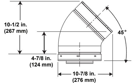
DVP45 (45° Elbow)
