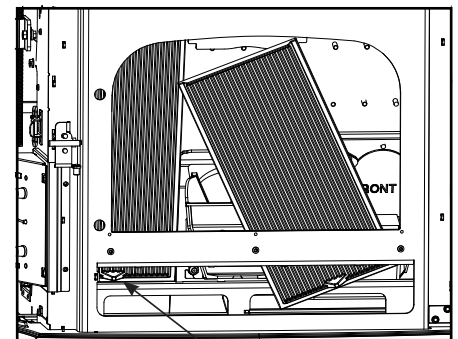
Figure 2.3a Lifting tab
