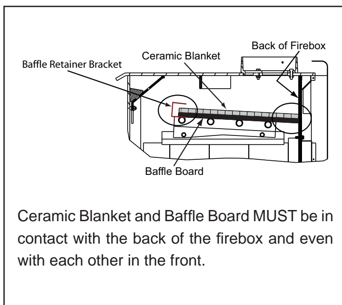
Figure 13.1 - Correct Baffle and Blanket Positions
