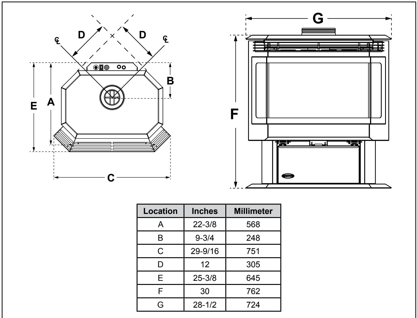
Figure 12.1 - Appliance Dimensions
