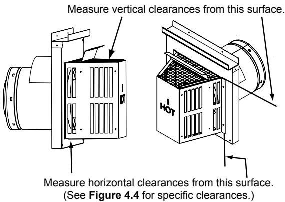
Figure 4.1 Termination Clearances
