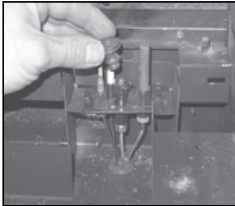
Figure 6.6 - Remove pilot hood and set aside. NOTE: Do not remove retaining clip from pilot hood.
