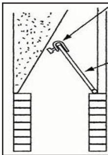
Figure 10 Damper Stop Clamp
