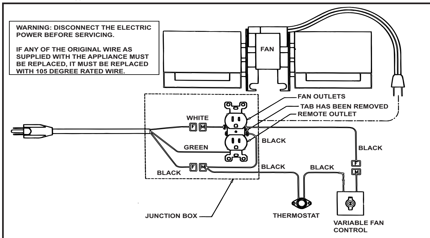
Wiring Diagram A
