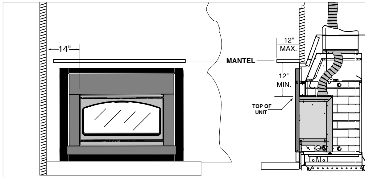
Diagram B - i30SE Clearances
