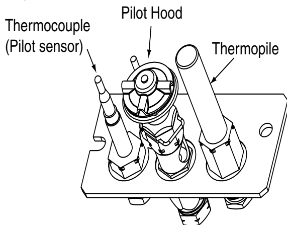
Figure 20 - Standing Pilot
