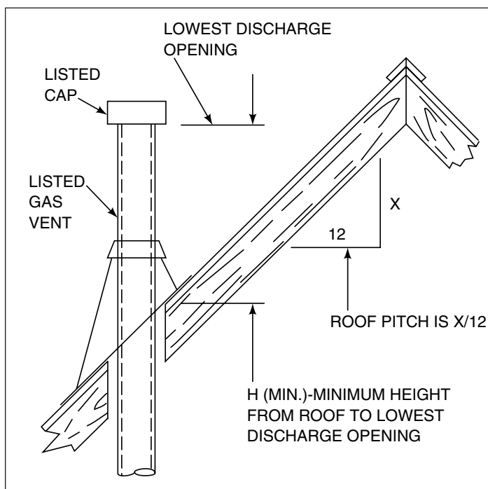
Figure 8 Termination Height
