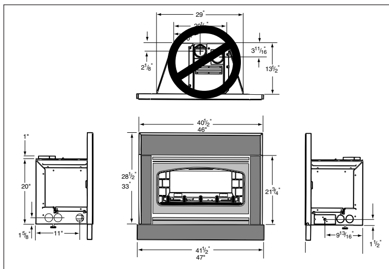
Diagram A - i30SE Dimensions
