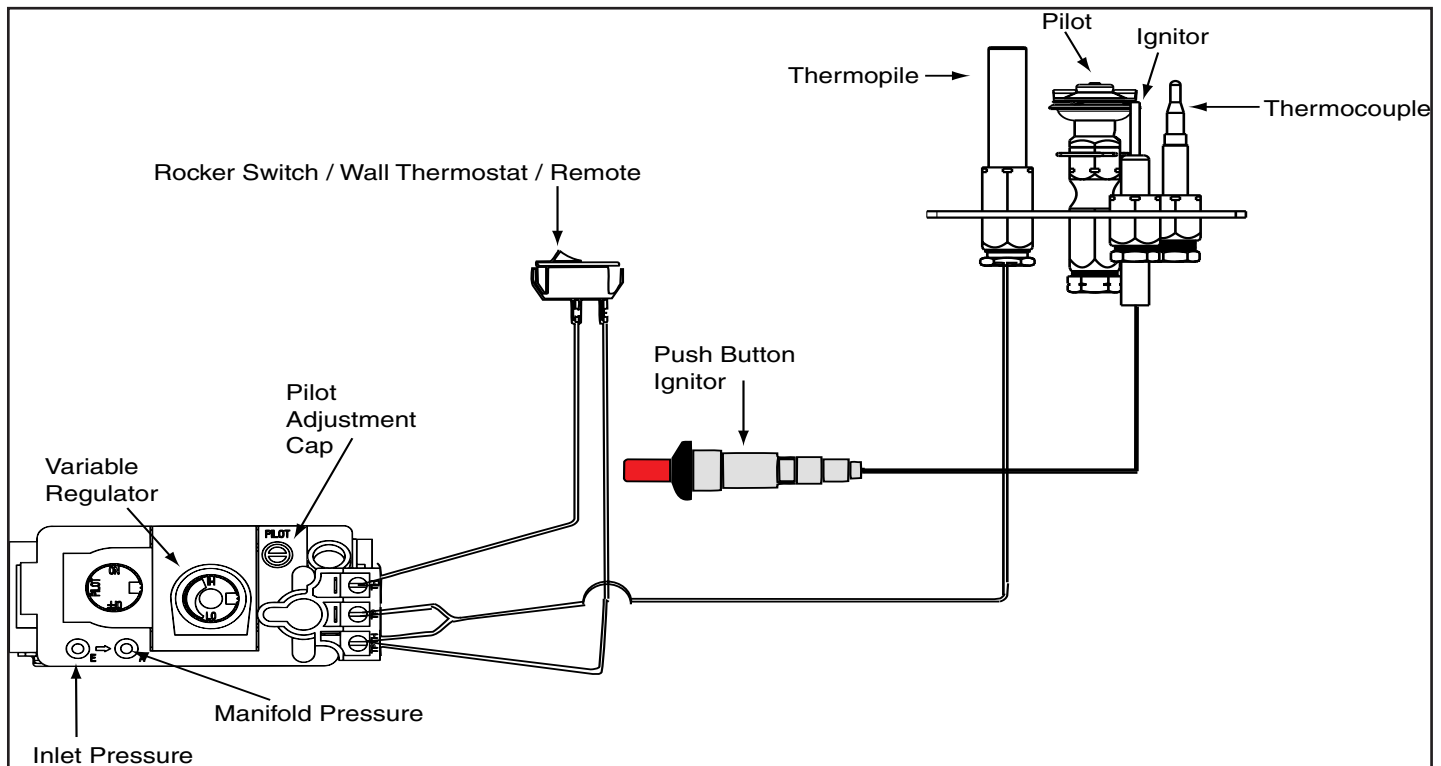
Wiring Diagram B
