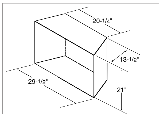
i30SE Minimum Firebox Opening
