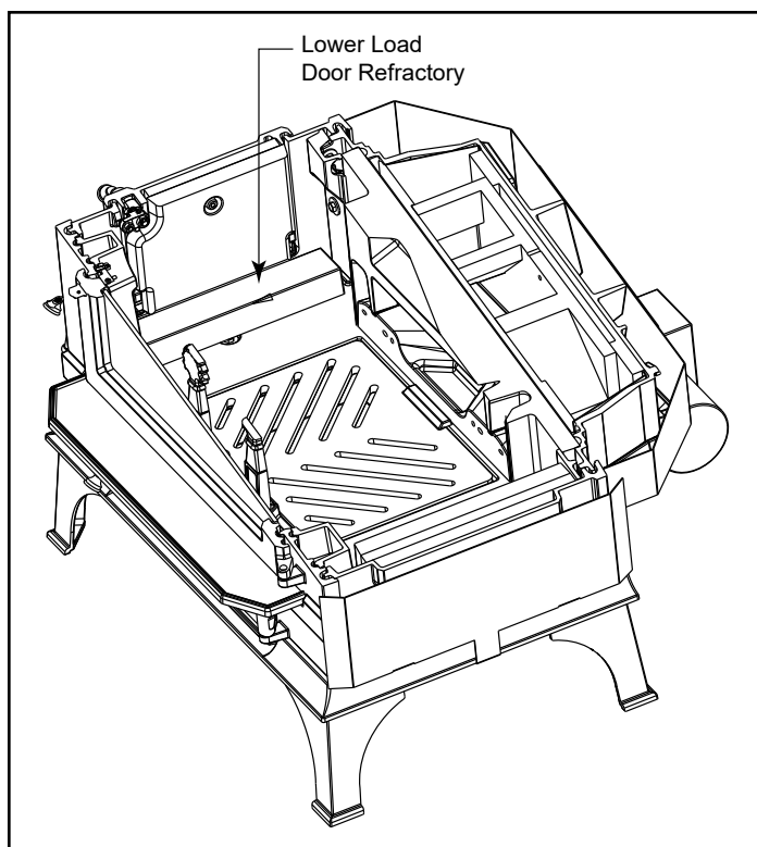
Figure 22 - Install lower load door refractory. (Cutaway view for clarification.)
