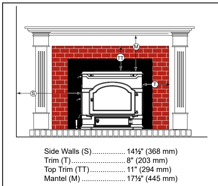
Figure 15 - Minimum clearances for fireplace installation. Recommended clearances must be maintained between stove and the surrounding combustible components.
