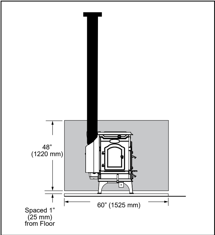
Figure 17 - Sidewall protection.
