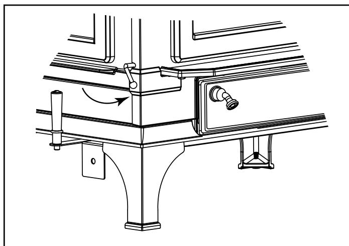
Figure 26 - Turn primary air control lever counterclockwise to close.
