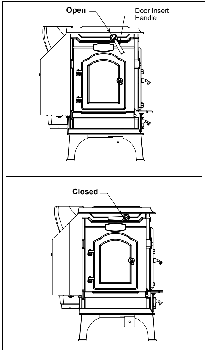
Figure 27 - Damper operating positions.
