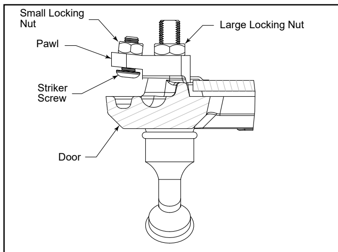
Figure 31 - Door latch adjustment.
