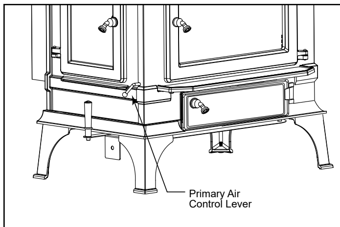
Figure 25 - Turn primary air control lever clockwise to open.
