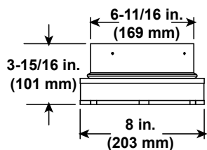
SL-2DVP Adapter
