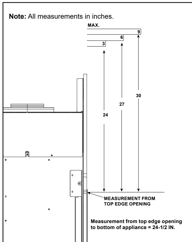
Figure 10.13 Minimum Vertical and Maximum Horizontal Dimensions of Combustibles - ECHEL60IN-C and ECHEL72IN-C
