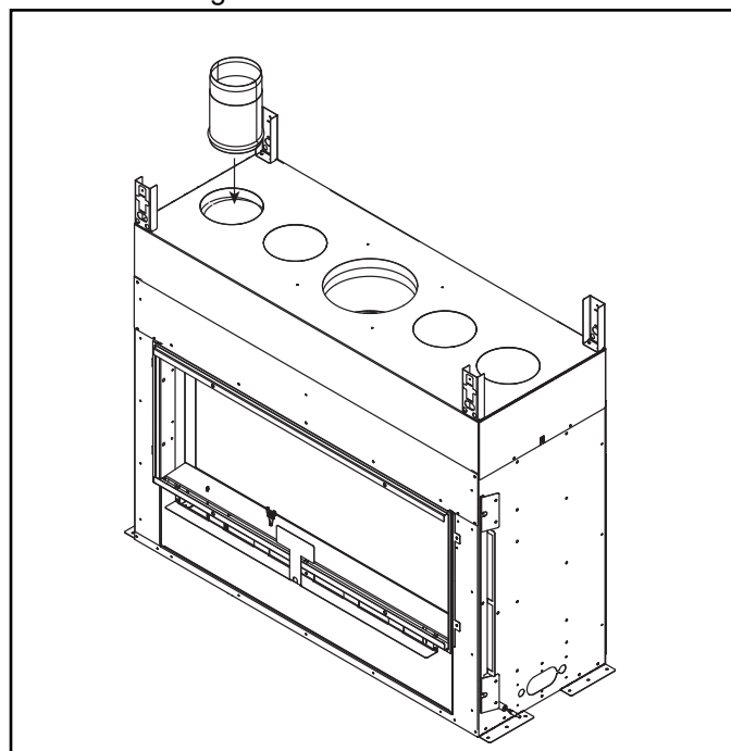
Figure 6.5 Heat-Zone-Gas Linear Adapter Collar
