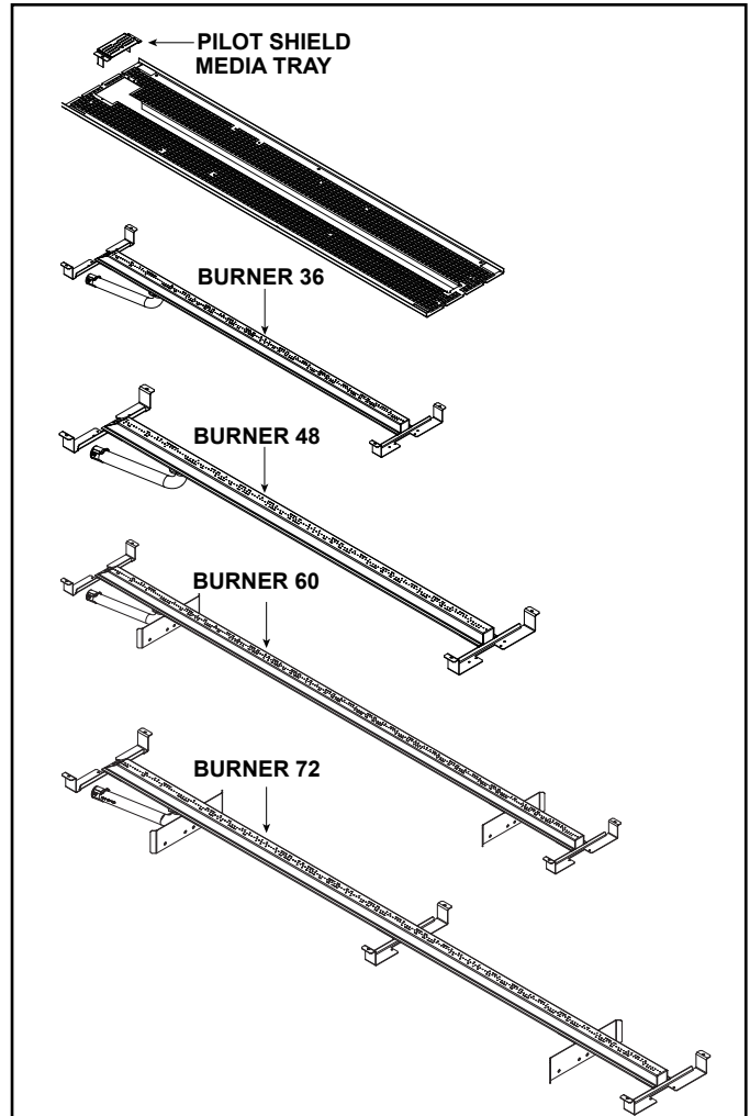
Figure 9.3 Media Tray with Burner and Pilot Shield
