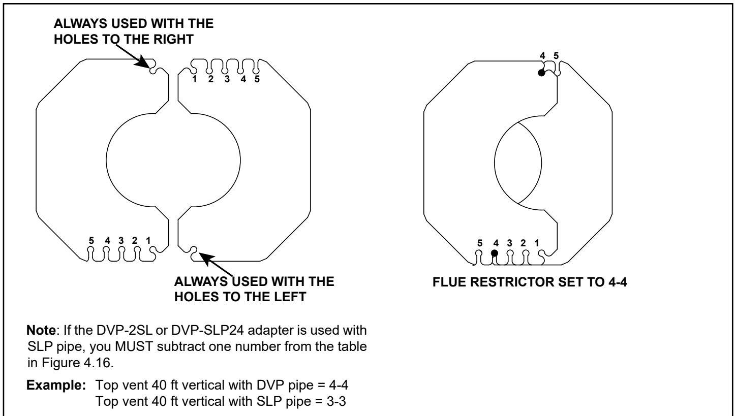
Figure 4.17 Setting the Flue Restrictor
