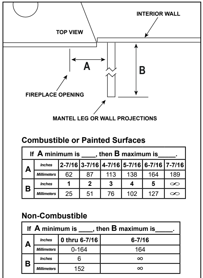
Figure 10.4 Clearances to Mantel Leg or Wall Projections (Acceptable on both sides of opening)
