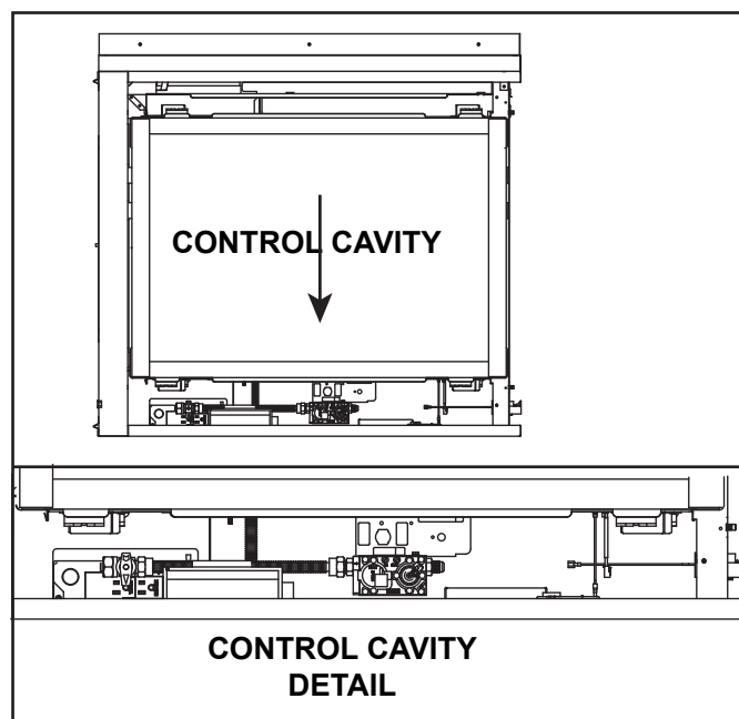
3.5 Control Cavity Location (PIER-36TR-IFT Shown)
