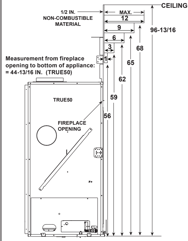
Figure 10.11 Combustible Mantel Allowance - TRUE-50
