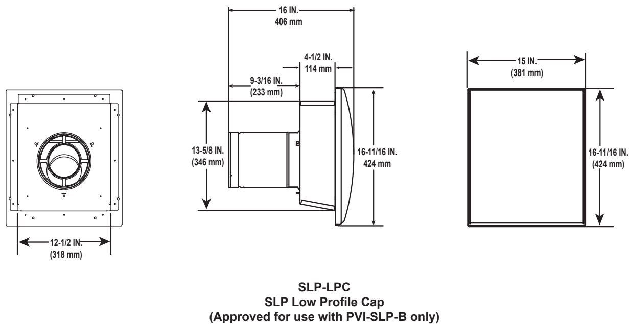
Figure 12.6 PVI-SLP-B Vent Components
