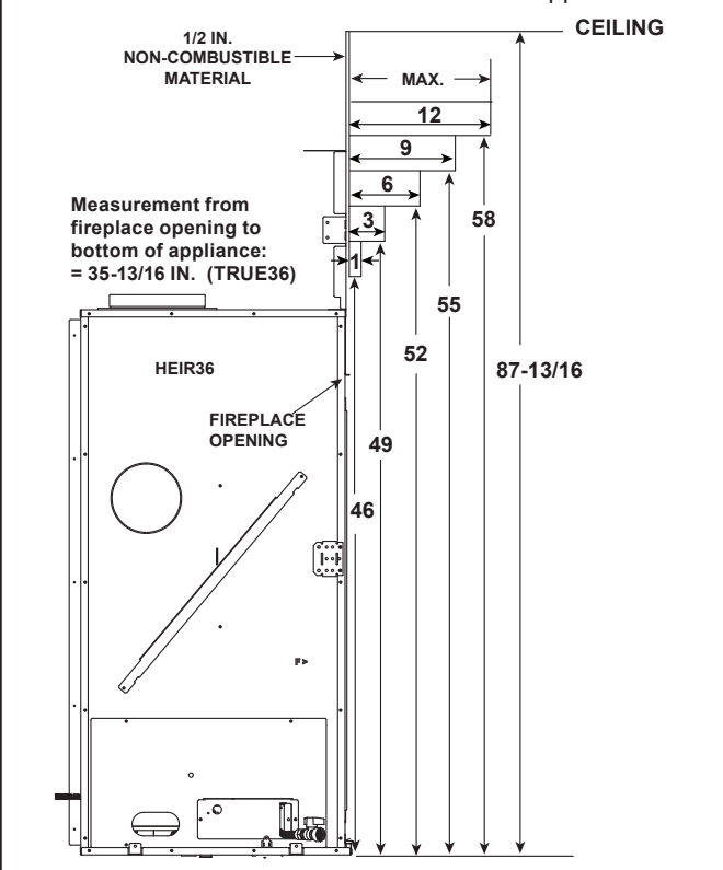
Figure 10.9 Combustible Mantel Allowance - TRUE-36
