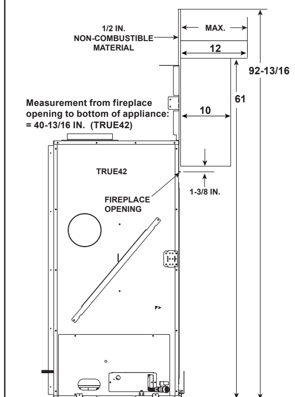
Figure 10.13 Non-Combustible Mantel Allowance - TRUE-42
