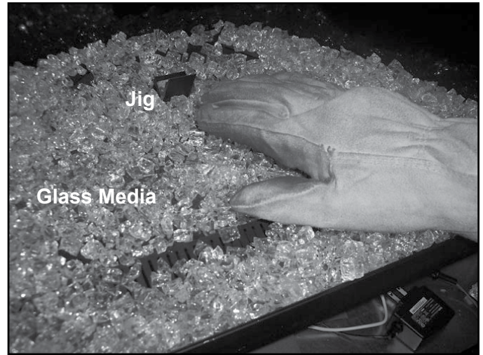
Figure 11.4 Place & Spread Glass Media
