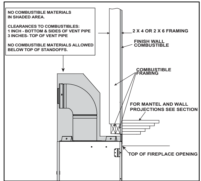
Figure 3.4 Clearances to Combustibles - Non-Combustible Zone
