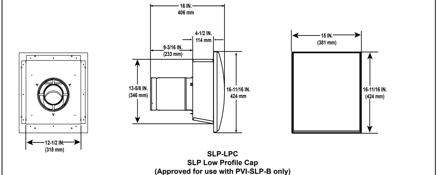
Figure 12.5 PVI-SLP-B Vent Components
