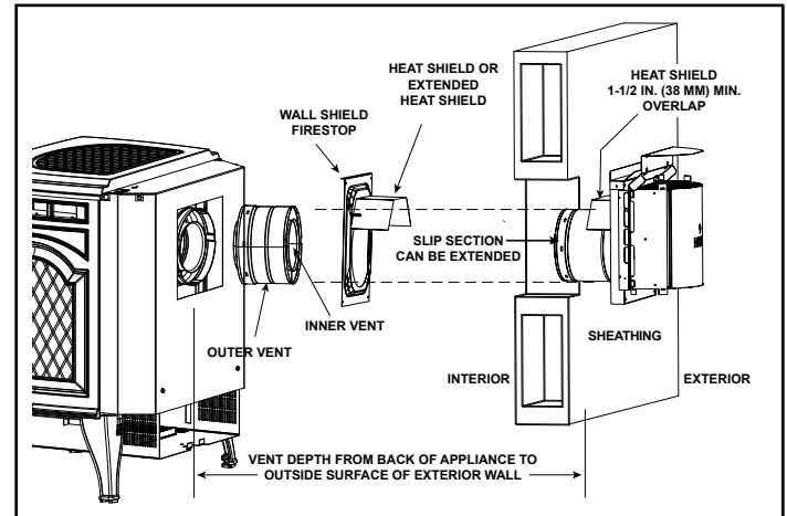
Figure 7.17 Venting through the wall
