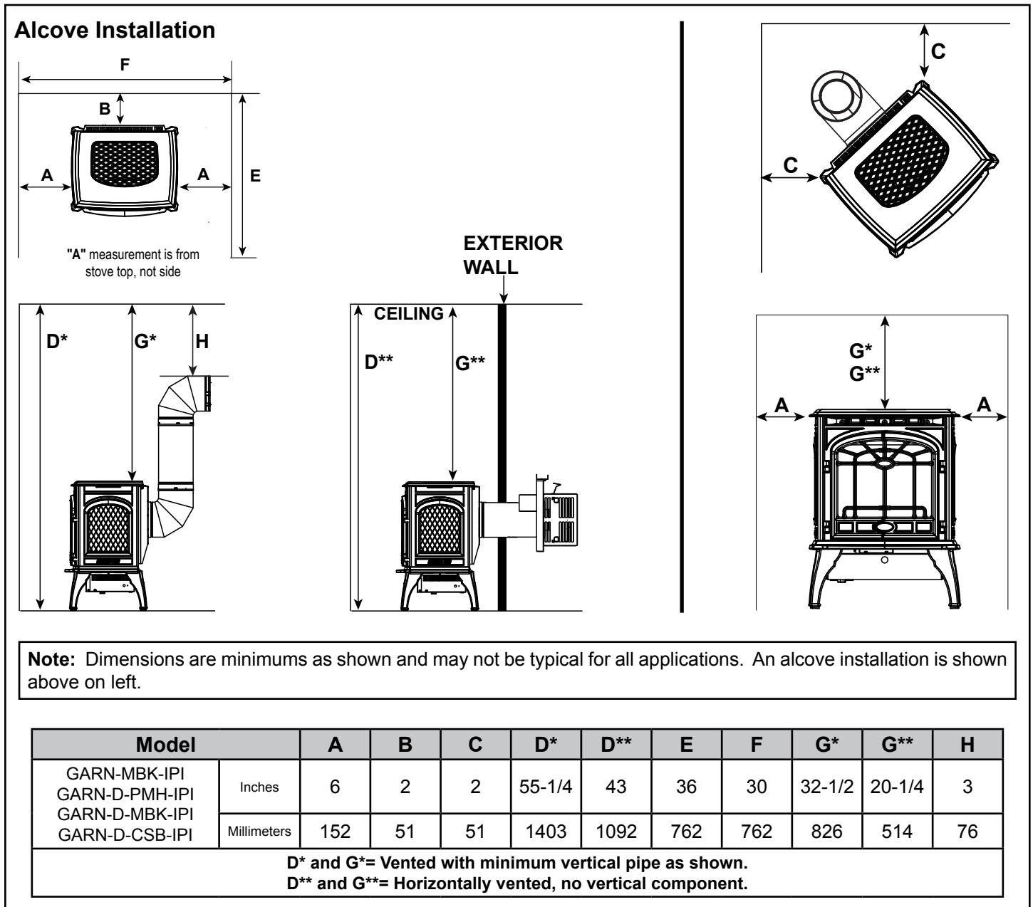
Figure 3.2 Appliance Locations
