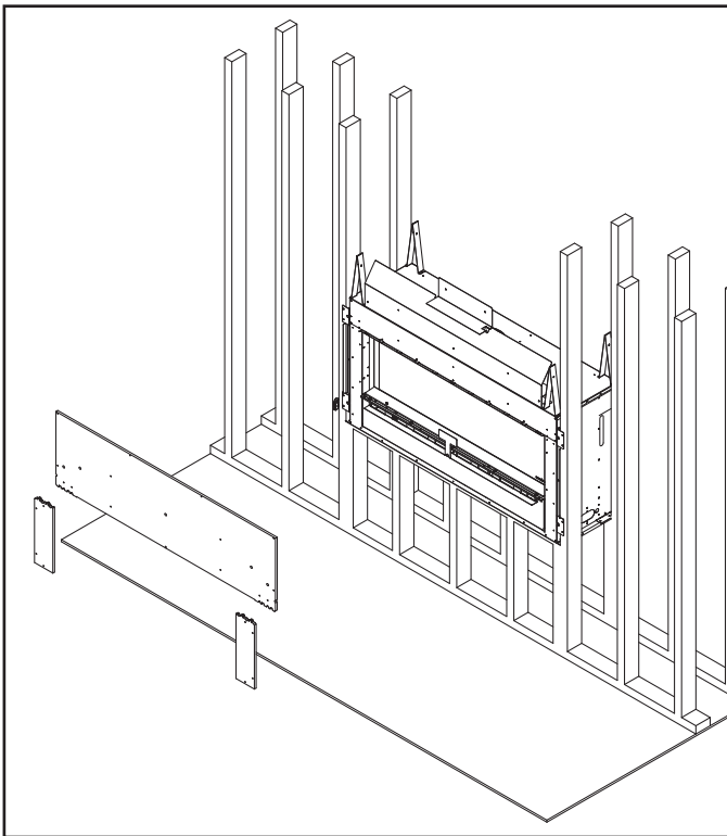
Figure 6.6 Install Factory-Included Non-Combustible Facing Material
