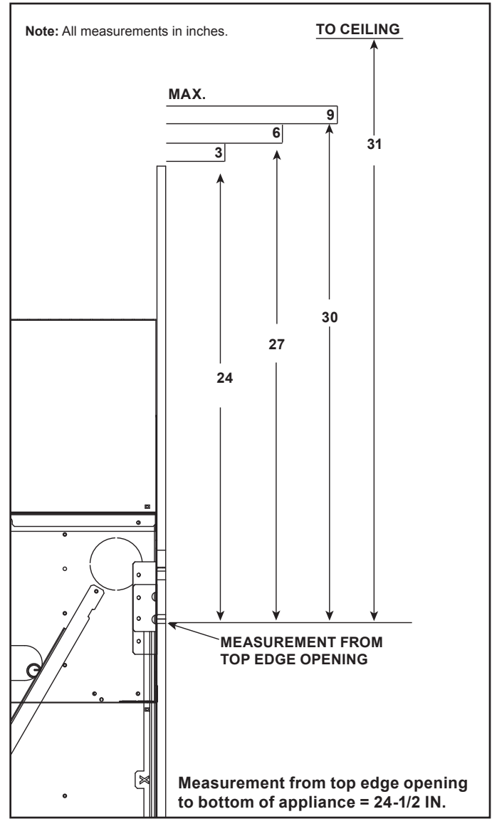
Figure 10.11 Minimum Vertical and Maximum Horizontal Dimensions of Combustibles - CRAVE7260 and CRAVE8472
