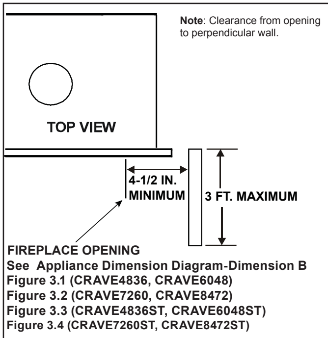
Figure 10.14 Mantel Leg or Wall Projections (Acceptable on both sides of opening)
