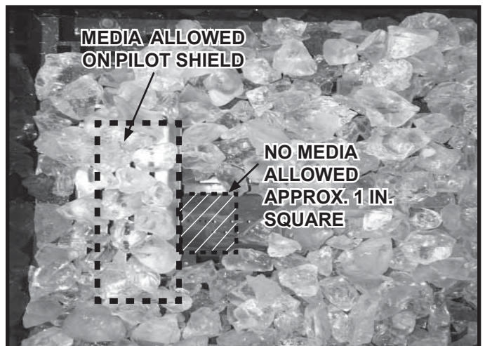
Figure 11.9. Pilot Shield Media installation.
