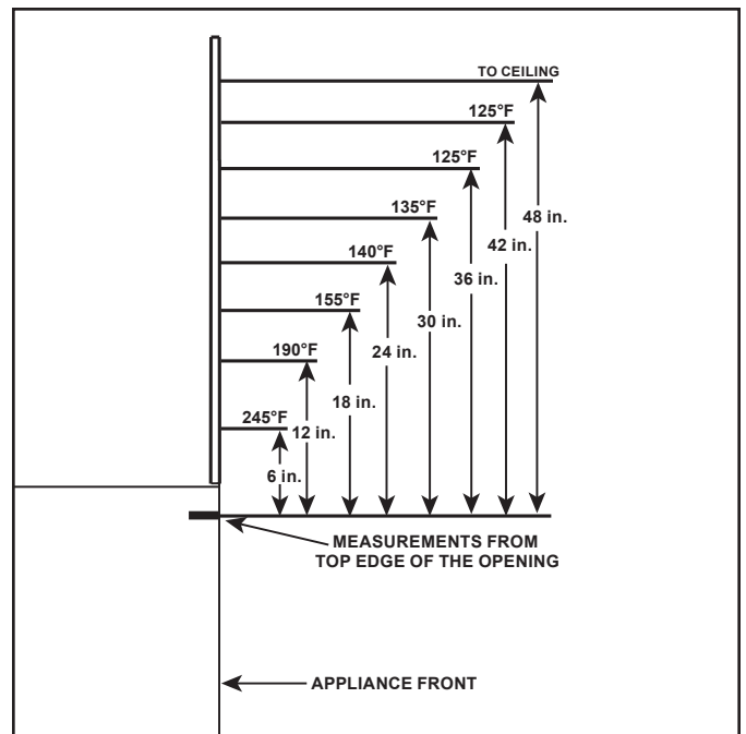
Figure 2.2. Wall Surface Temperatures Above Appliance (GRAVE7260/CRAVE7260ST/CRAVE8472/CRAVE8472ST)
