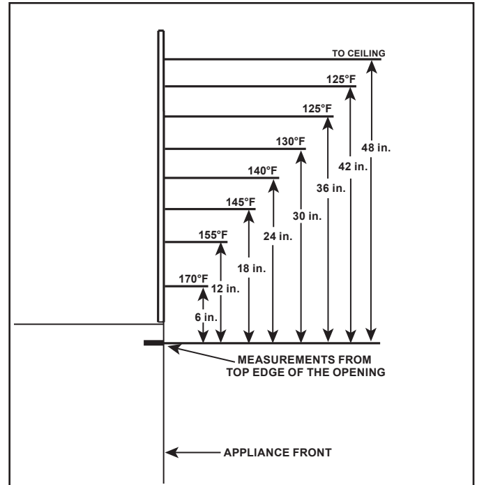
Figure 2.1. Wall Surface Temperatures Above Appliance (GRAVE4836/CRAVE4836ST/CRAVE6048/CRAVE6048ST)
