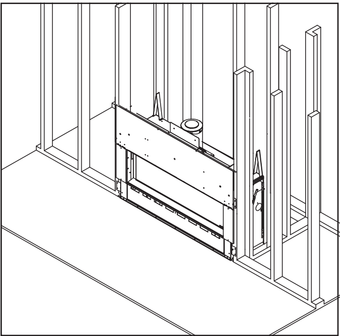
Figure 3.12 Floor Protection
