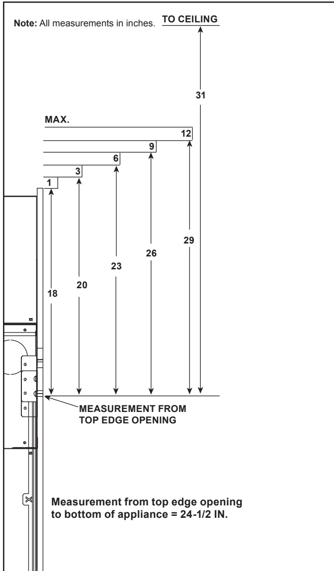
Figure 10.10 Minimum Vertical and Maximum Horizontal Dimensions of Combustibles - CRAVE4836 and CRAVE6048
