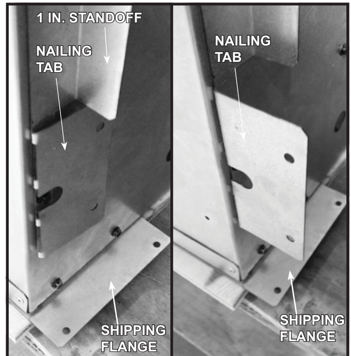
Figure 6.4 Nailing Tabs Shipping Position
