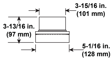
SL-2DVP Adapter
