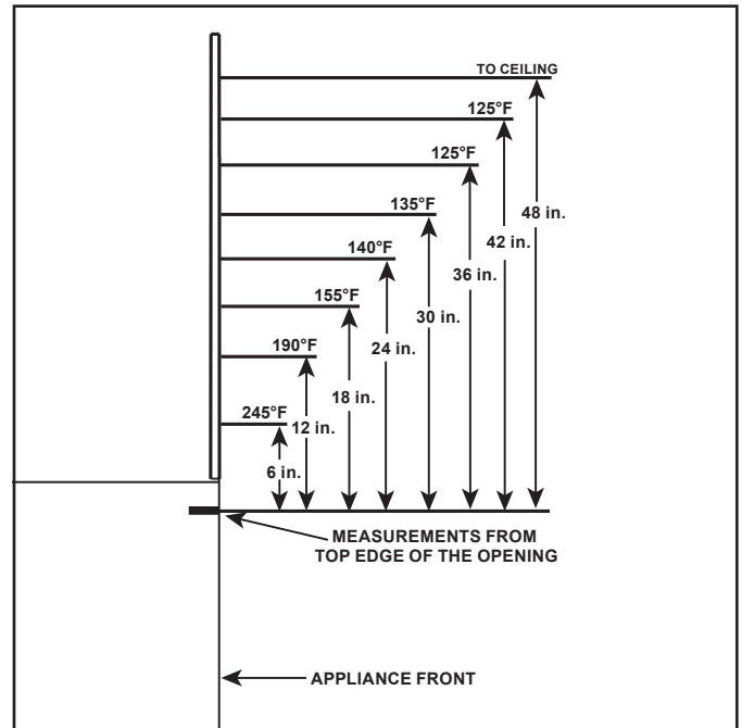
Figure 3.4. Wall Surface Temperatures Above Appliance (MEZZO60/MEZZO60ST/MEZZO72/MEZZO72ST)
