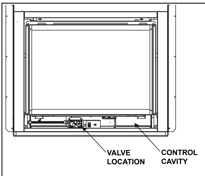
Figure 3.4 Control Cavity/Valve Location
