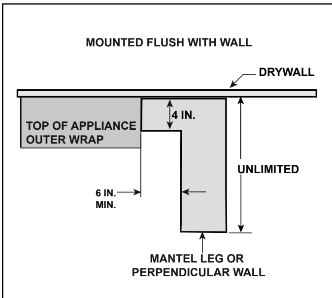
Figure 10.6 Non-Combustible Mantel Leg or Wall Projections (Acceptable on both sides of outer wrap)
