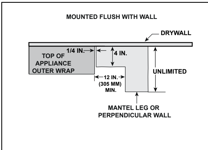
Figure 10.5 Combustible Mantel Leg or Wall Projections (Acceptable on both sides of outer wrap)
