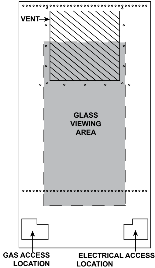
Figure 6.5 Corrugated Template Dimensions - ION-V7
