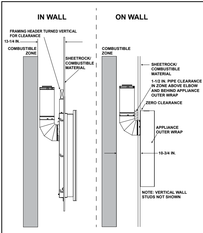
→ Figure 3.9 Clearance Requirements
