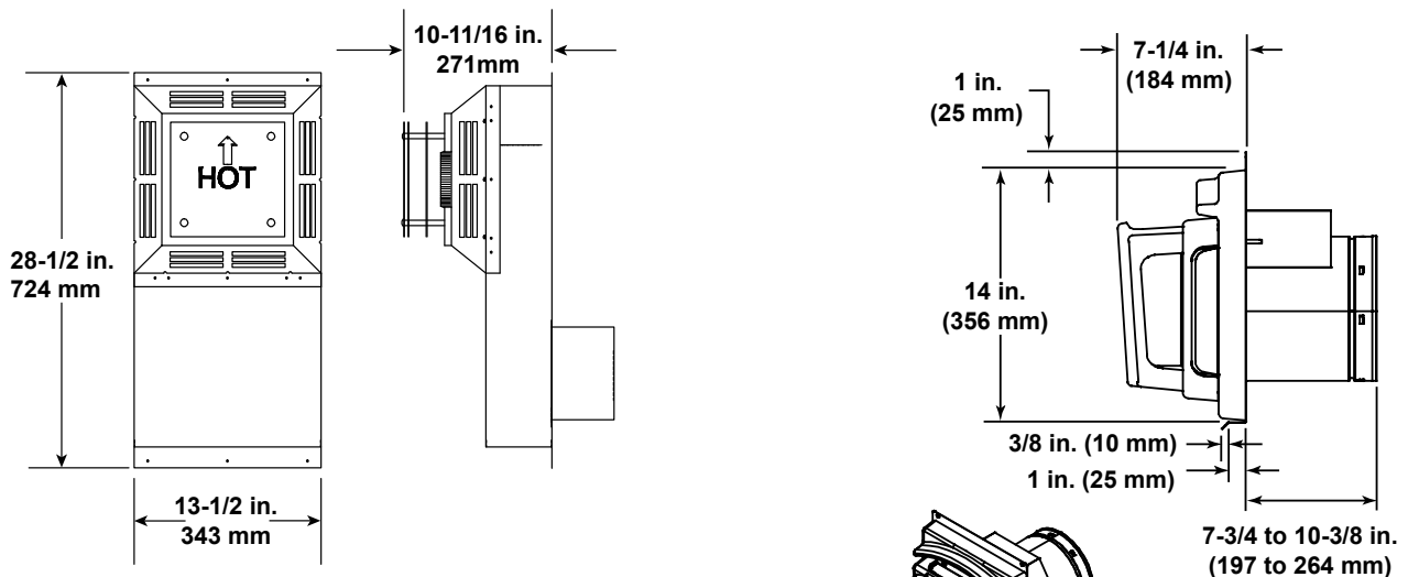
DVP-FBHT Horizontal Termination Cap
