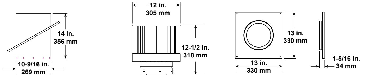
SLP-CCS-BK Cathedral Ceiling Support Box-Black
