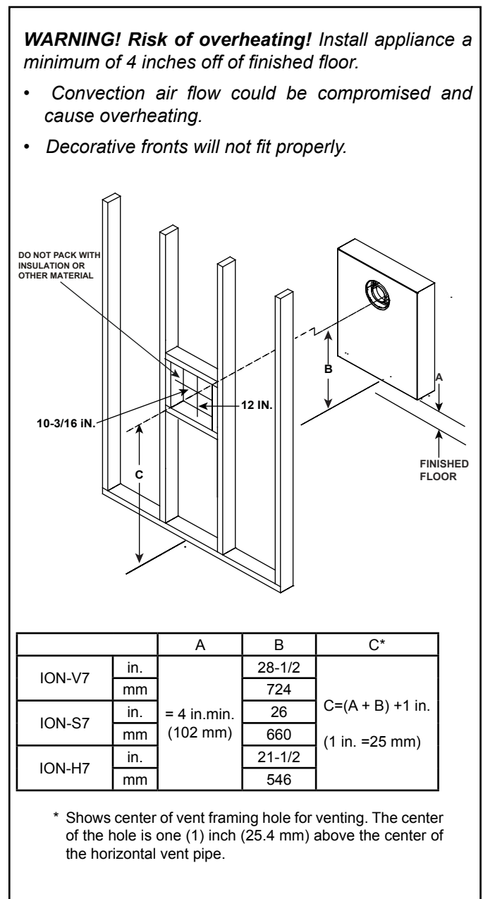
Figure 5.2 Wall Penetration
