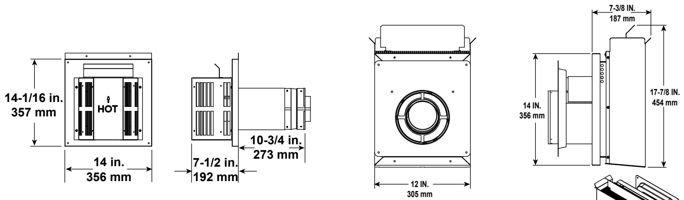
SLP-FLEX-TRAP Horizontal Termination Kit
