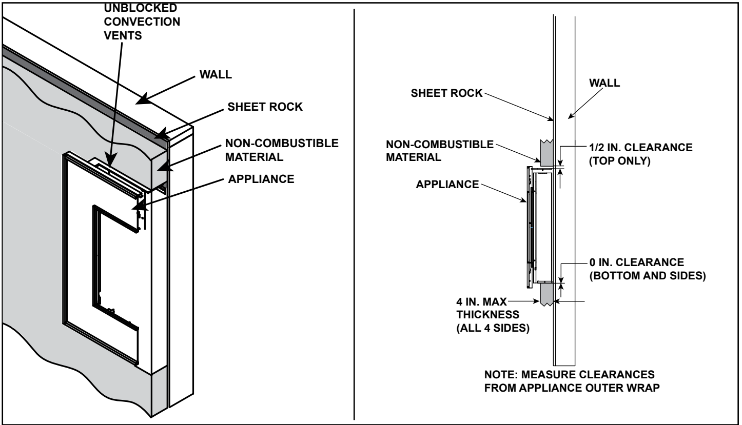
→ Figure 10.3 Non-Combustible Facing Diagram
