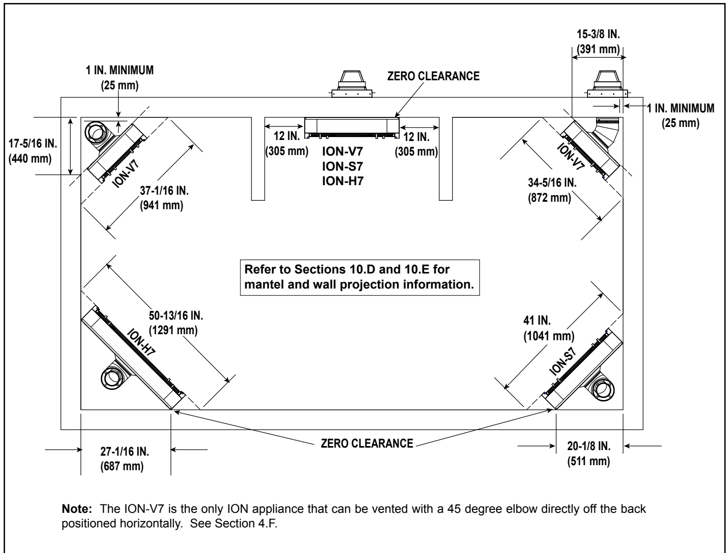
Figure 3.6 Appliance Locations
