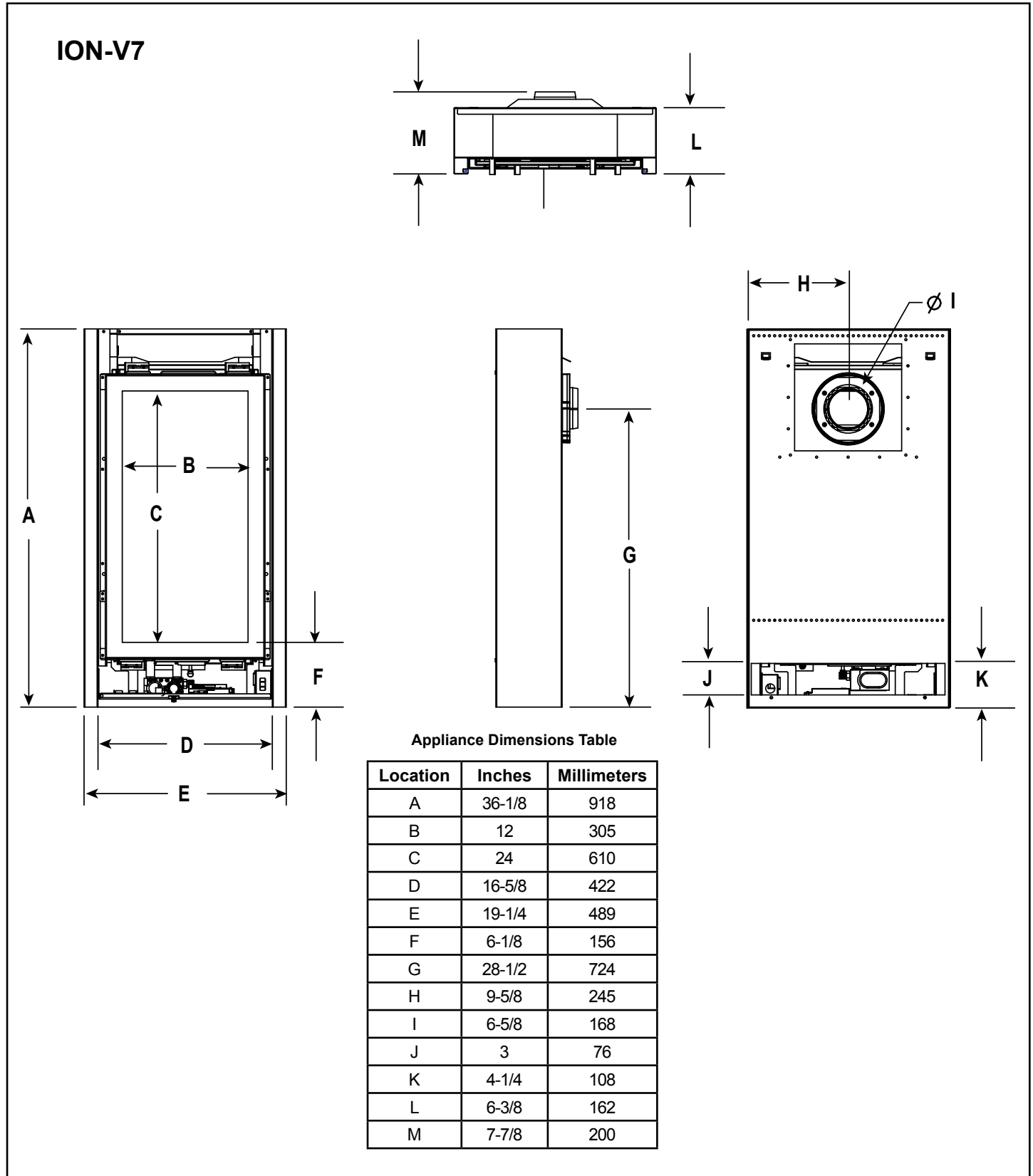
Figure 3.1 Appliance Dimensions - ION-V7
