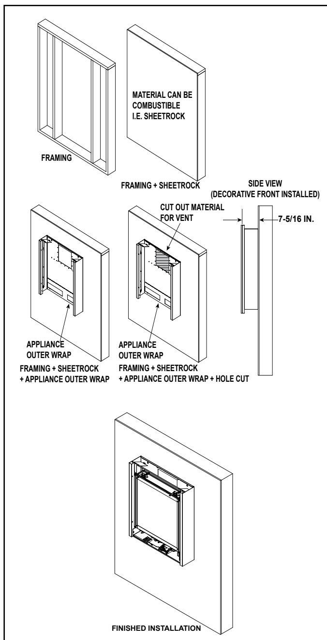
→ Figure 2.1 On-Wall Installation Method
