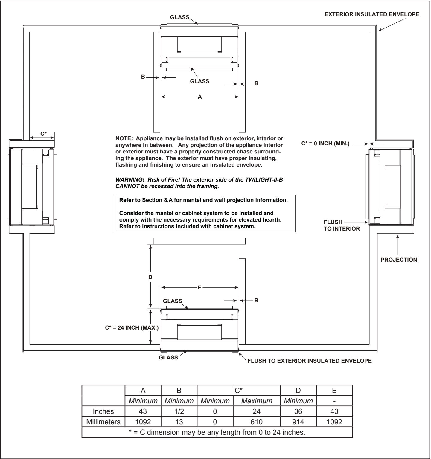
Figure 3.2 Appliance Locations
