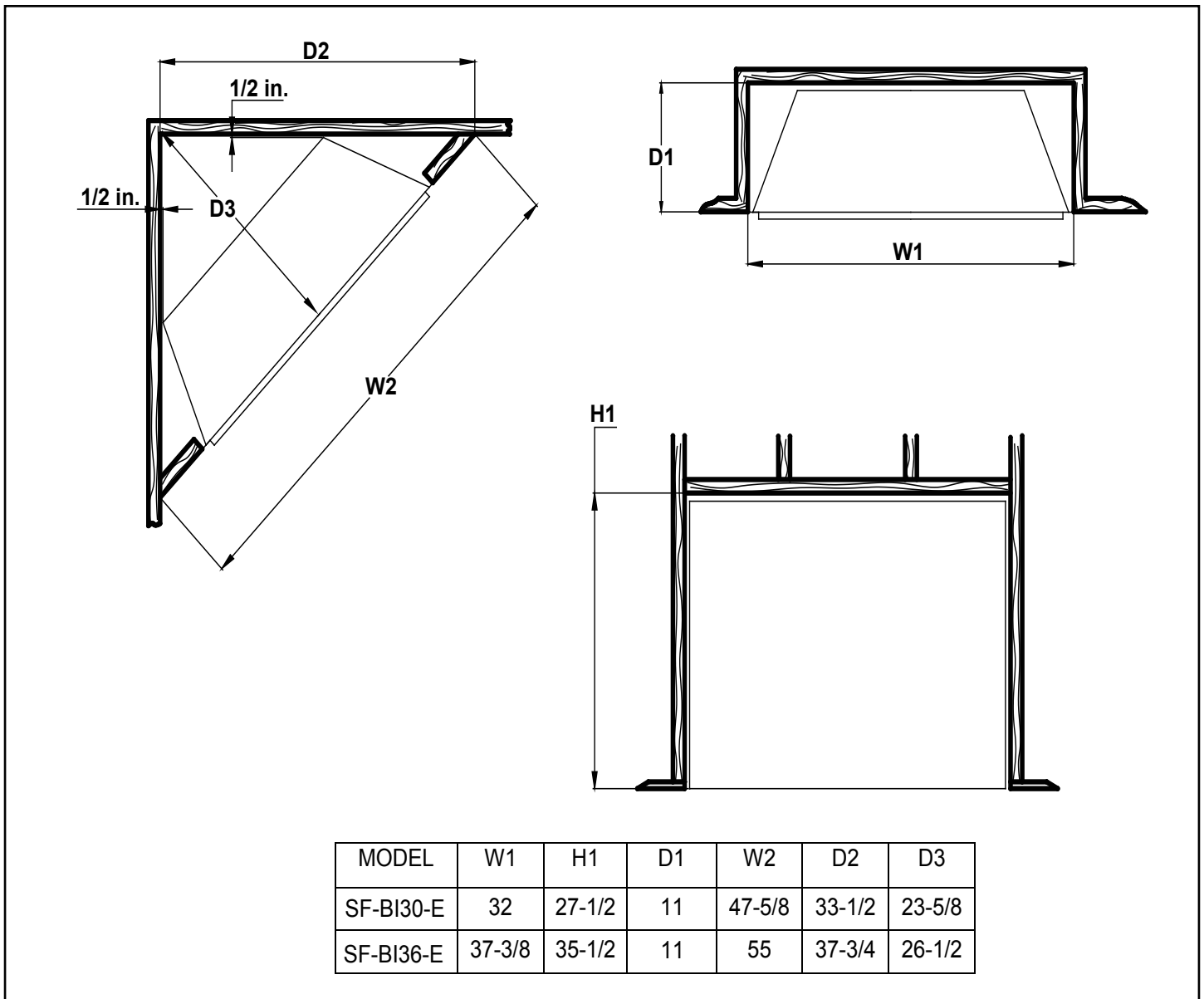
Figure 4.1 Clearance Requirements
